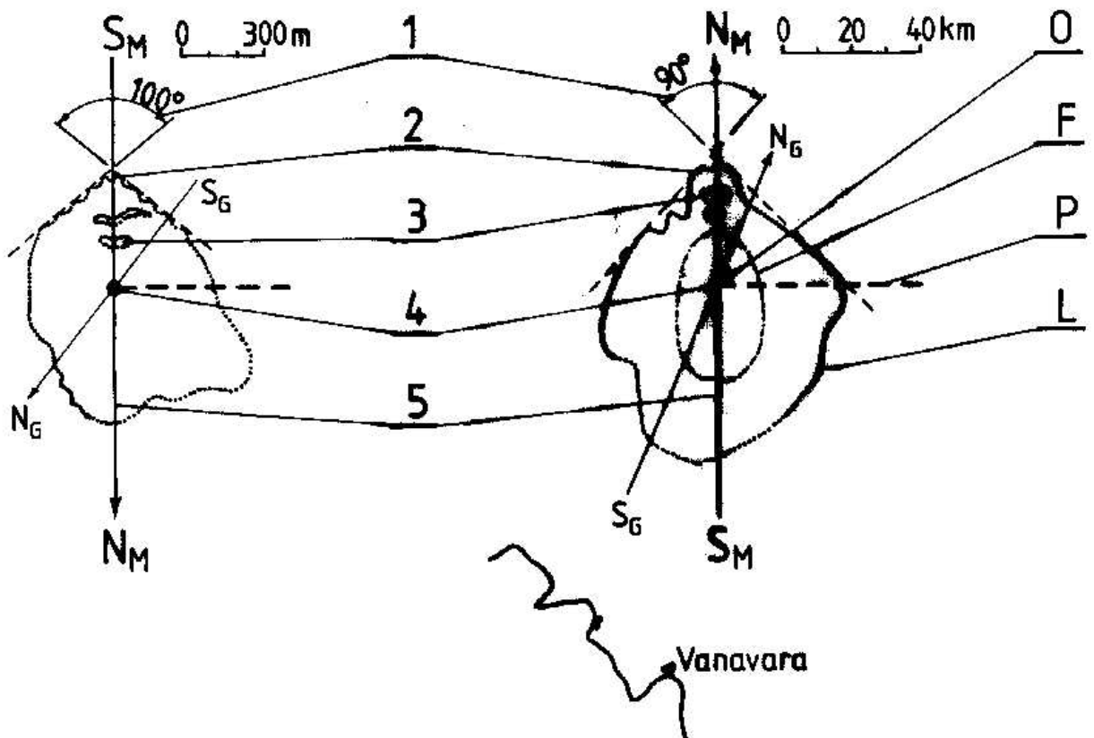
Fig. O5. The illustration of similarities existing between the configuration of the Tapanui Crater and that of the Tunguska blast site. The presence of such close similarities certify that the origin of both sites is analogous, i.e. from a powerful near-ground (aerial) explosion. Notice the evident correspondence (labelled 1 to 5) in: (1) the relationship between the apical angle of triangular entries to both sites and their distance from the nearest magnetic pole of Earth (i.e. at the moment of explosion the Tapanui Crater was located much closer to the magnetic pole than the Tunguska Site, thus its apical angle is also much wider), (2) the manner explosion shockwaves entered the ground, (3) the breaking points of the explosion shockwaves (which in Tunguska swirled tree trunks, whereas in Tapanui formed large sand dunes), (4) the location of the centre of explosions and the paths followed priori by both vehicles, (5) magnetic meridian orientation of the sites, etc. Symbols: S G /N G - geographic south-north direction, S M /N M - magnetic south-north direction.
