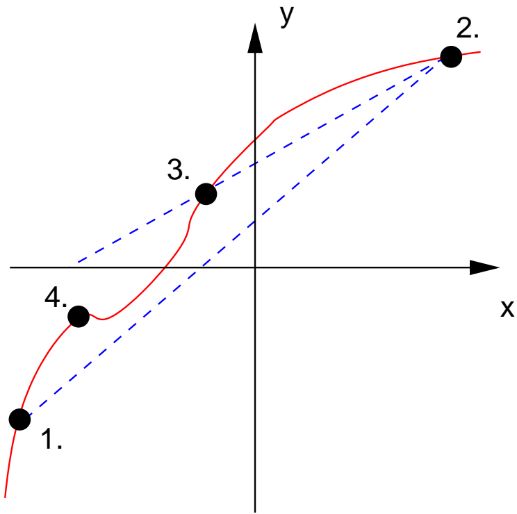
Secant Method
