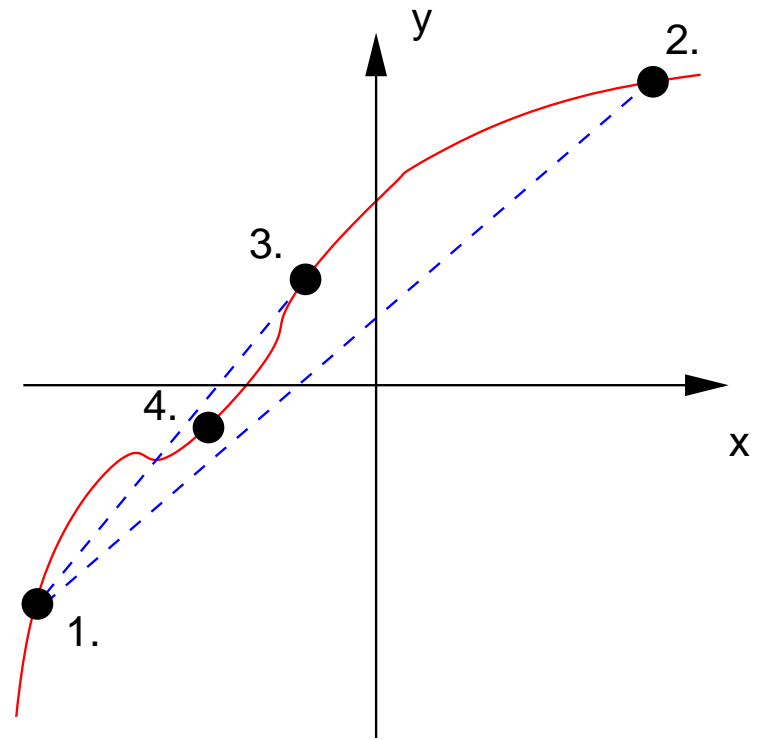
Regula Falsi Method
