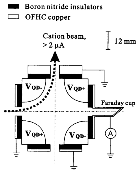
FIG. 4. Quadrupole deflector cooled to 77 K during experiments: Boron nitride insulator disks (1.5 in. diameter) and OFHC copper electrodes were used to simultaneously maximize electrical insulation and thermal conductivity.
