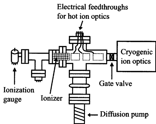
FIG. 1. Ion beam vacuum chamber (ionizer and hot ion optics region).
