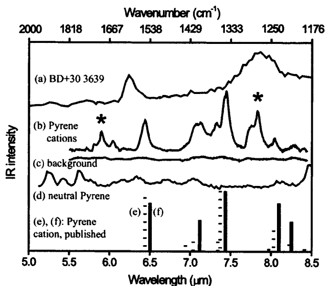
FIG. 7. SPIRE spectrum of gas-phase pyrene cations ( C_{16}H_{10}^+ and etc.) in the 5.5–8.5 \mu\text{m} region when the pyrene vapor pressure was relatively low ( 1.0 \times 10^{-2} Torr): Trace (b) is the observed SPIRE spectrum of gas-phase pyrene cations with the background subtracted, corrected for monochromator (filters, mirrors, a diffraction grating and a detector) throughput and its intensities are normalized. Trace (c) is the background spectrum. Trace (d) is the gas-phase SPIRE spectrum of neutral pyrene reported previously (see Ref. 4). The IR absorption spectra for the pyrene cation ( C_{16}H_{10}^+ ) are shown in (e) and (f) as stick diagrams for comparison. The SPIRE spectrum in (b) matches well with both the matrix absorption (see Ref. 7) spectrum (e) and the gas-phase absorption (see Ref. 12) spectrum (f), except for the bands near 5.8–6.1 and 7.7–7.8 \mu\text{m} , marked with asterisks. The UIR spectrum from a planetary nebula, BD+30°3639 in this region is also shown in (a) for comparison.
