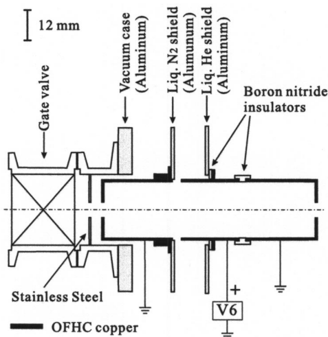
FIG. 3. Einzel transfer lens cooled to 77 K during experiments.
