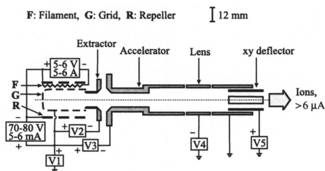
FIG. 2. The SPIRES ion gun and hot ion optics: Vaporized pyrene molecules are ionized by 70–80 eV electrons, yielding an ion beam with ion currents of at least 6 \mu\text{A} and 1 keV beam energy at the entrance aperture of the cryogenic ion optics system.
