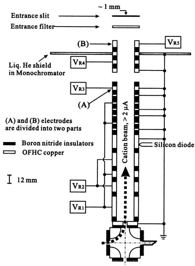
FIG. 5. Reflectron cooled below 77 K during experiments: The last ring of stack [R4, R5, (B) electrodes and their electrical isolators, boron nitrides] are contacting with Liq. He shield cooled to liquid He. A series of boron nitride insulator disks (1.5 in. diameter) are arranged between OFHC copper ring electrodes (1.5 in. diameter) to simultaneously maximize electrical insulation and thermal conductivity.
