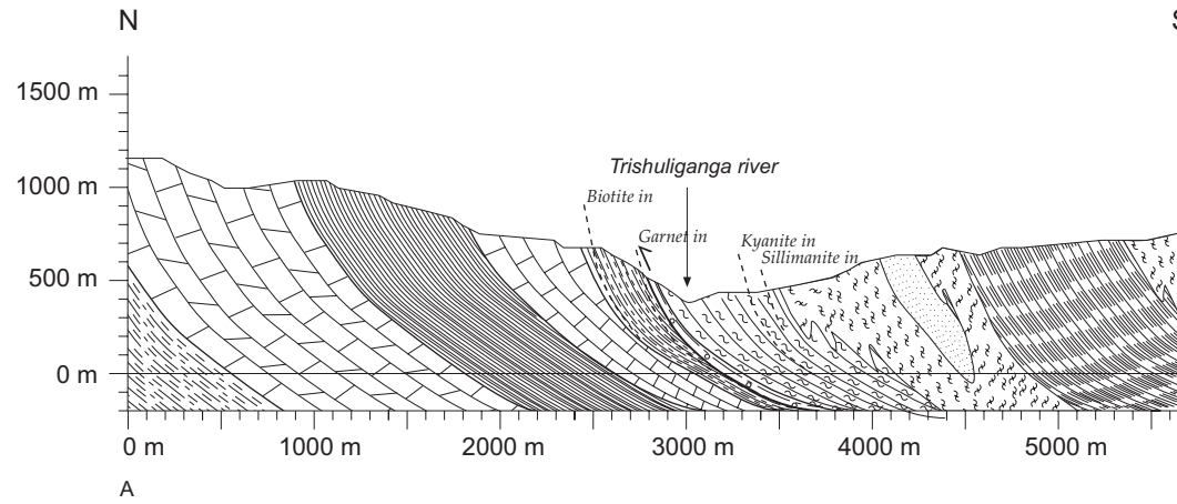
Cross-section along A-B
