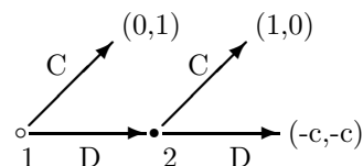
図 1: Threat Game
