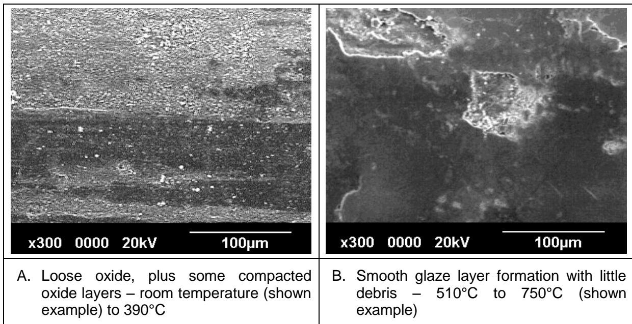
Fig. 3: SEM images of Nimonic 80A wear surfaces after sliding at 0.314 m.s -1 against a Stellite 6 counterface at room temperature and 750°C
