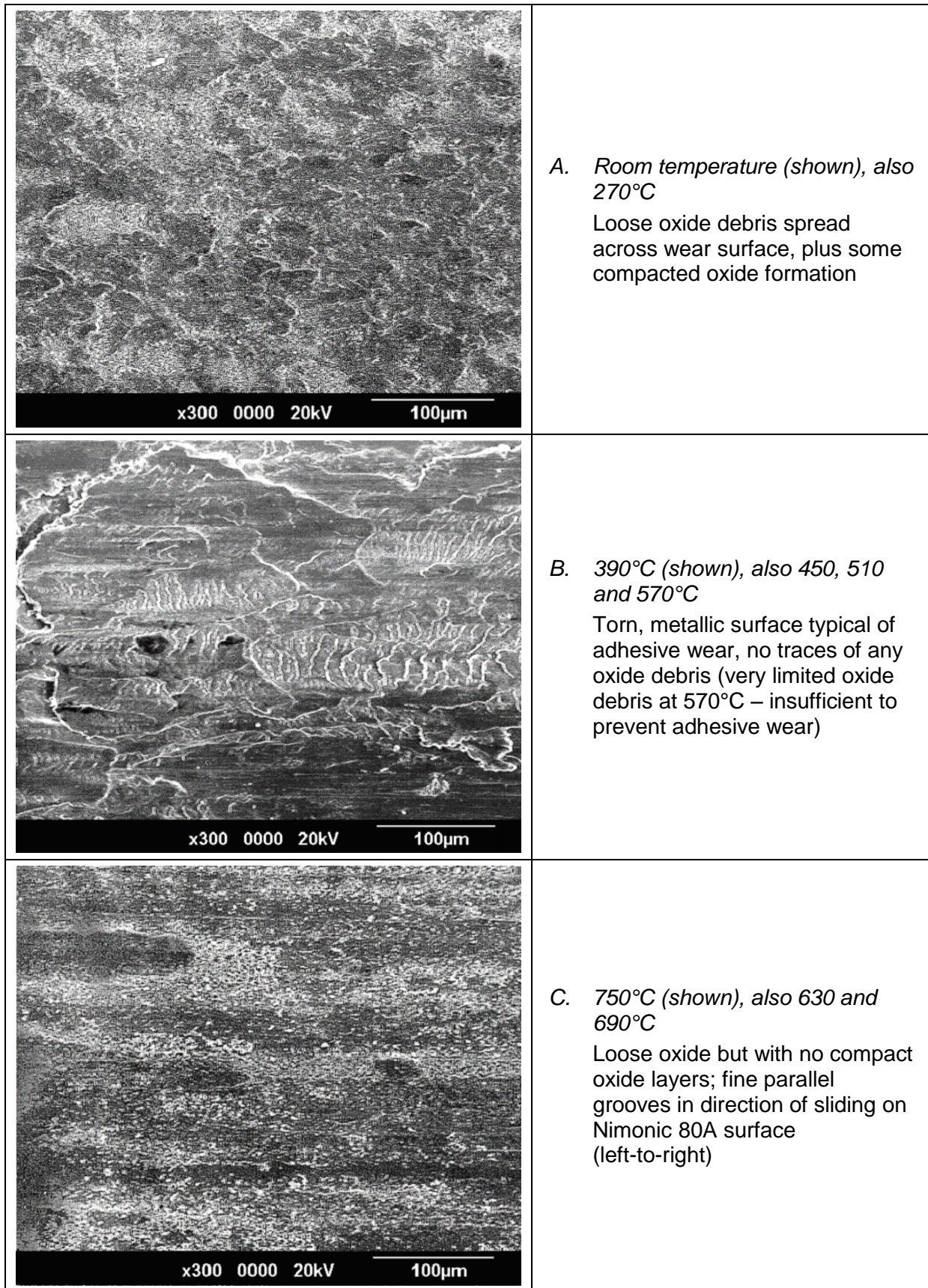
Fig. 9: SEM images of Nimonic 80A wear surfaces after sliding at 0.905 \text{ m}\cdot\text{s}^{-1} (sliding distance 4,522 m) against a Stellite 6 counterface at room temperature, 390°C and 750°C
