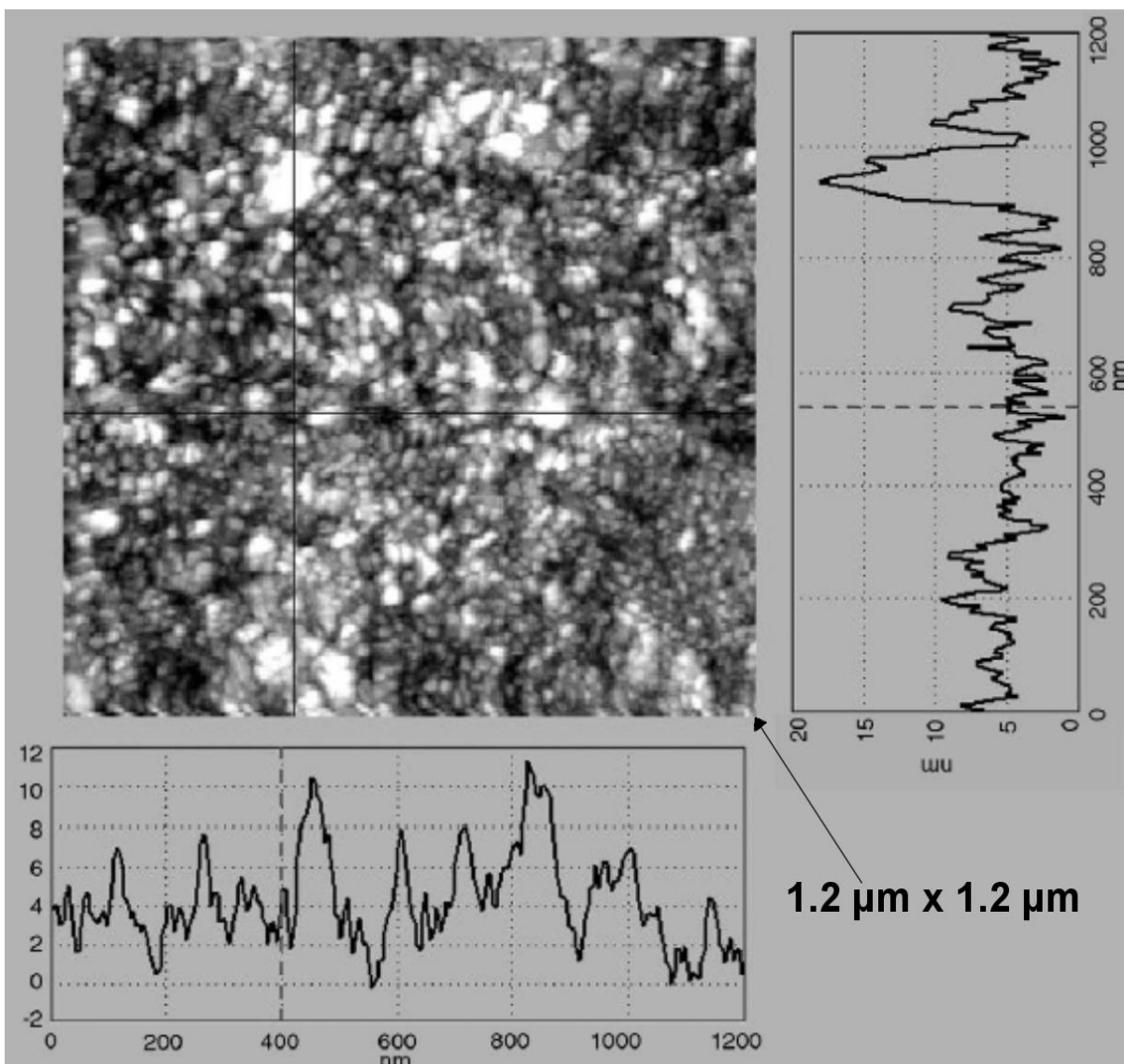
Fig. 7: STM surface line profile results on the glaze layer formed on Nimonic 80A at 0.314 \text{ m.s}^{-1} and 750^\circ\text{C}
