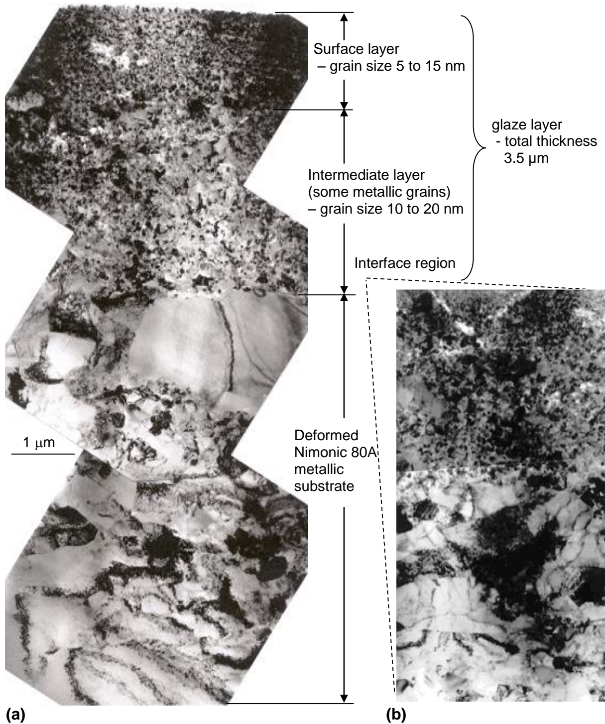
Fig. 5: Nano-scale characterisation of glaze layers formed at 0.314 \text{ m.s}^{-1} and 750^\circ\text{C} showing TEM bright field images of (a) a wear-induced polycrystalline glaze layer plus substrate deformation and (b) the interface of the glaze layer and deformed substrate
