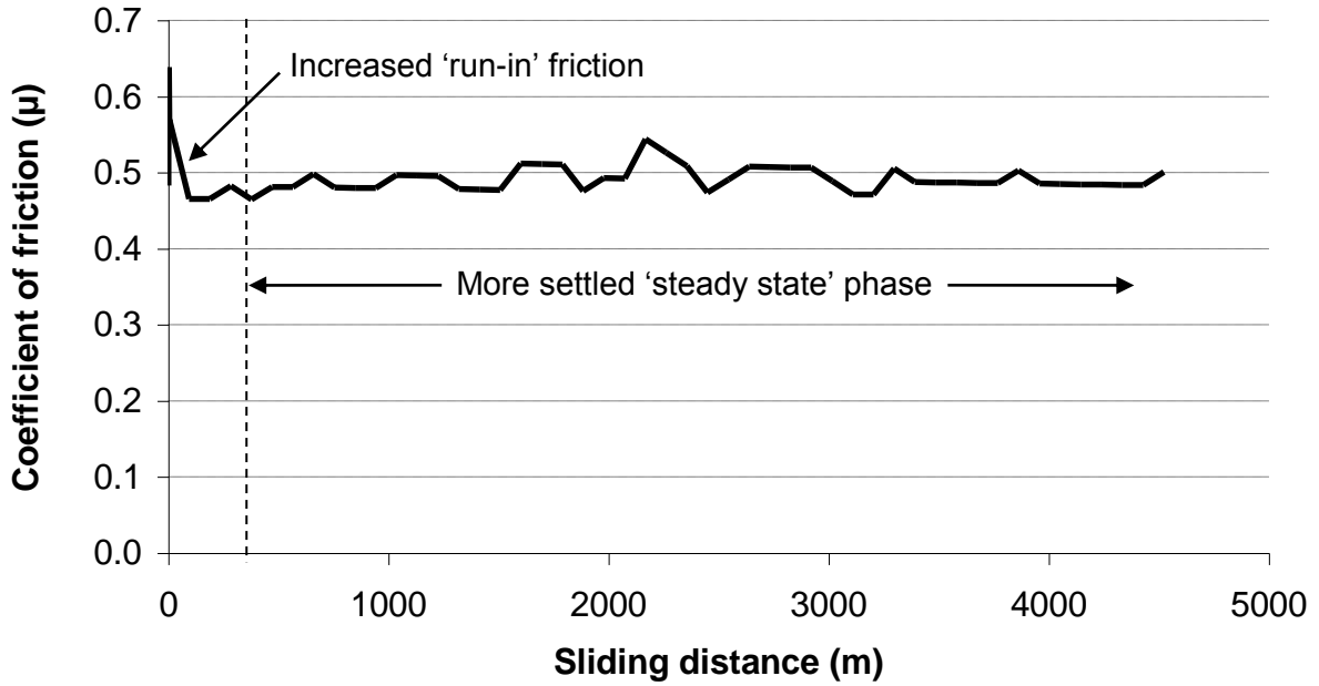
Fig. 4: Coefficient of friction versus time for Nimonic 80A versus Stellite 6 at 0.314 \text{ m.s}^{-1} and 750^\circ\text{C}
