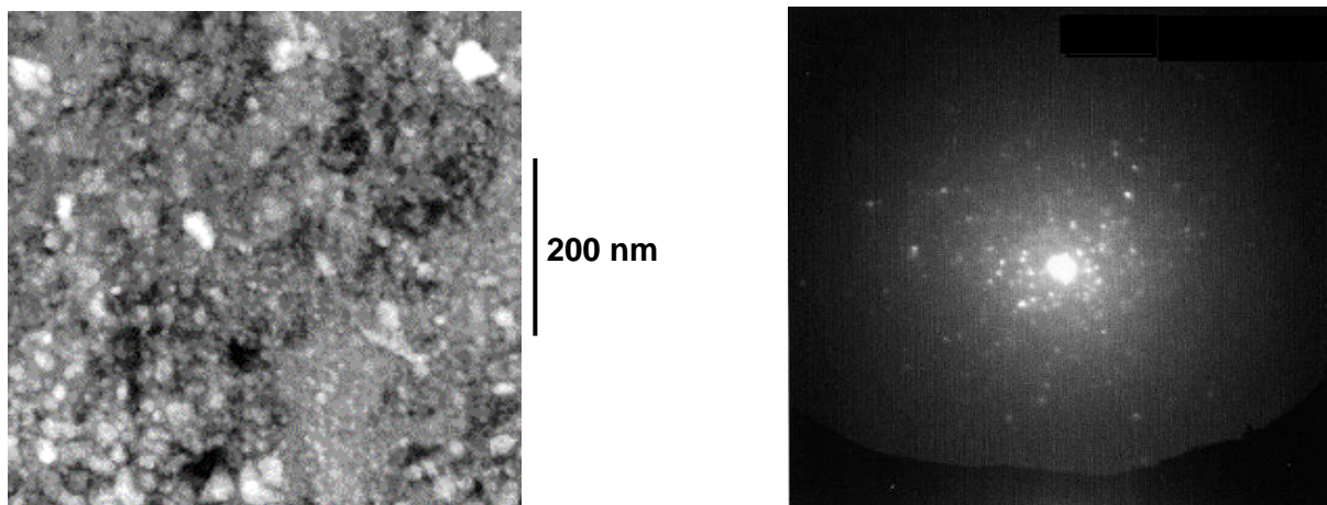
Fig. 11: TEM image (left) of a nano-crystalline compact oxide layer formed by sliding of Nimonic 80A versus Stellite 6 at 0.314 m.s -1 and 20°C [30]. SAD (right) shows only the presence of small randomly oriented grains in the glaze layer near the interface with the Nimonic 80A substrate.
