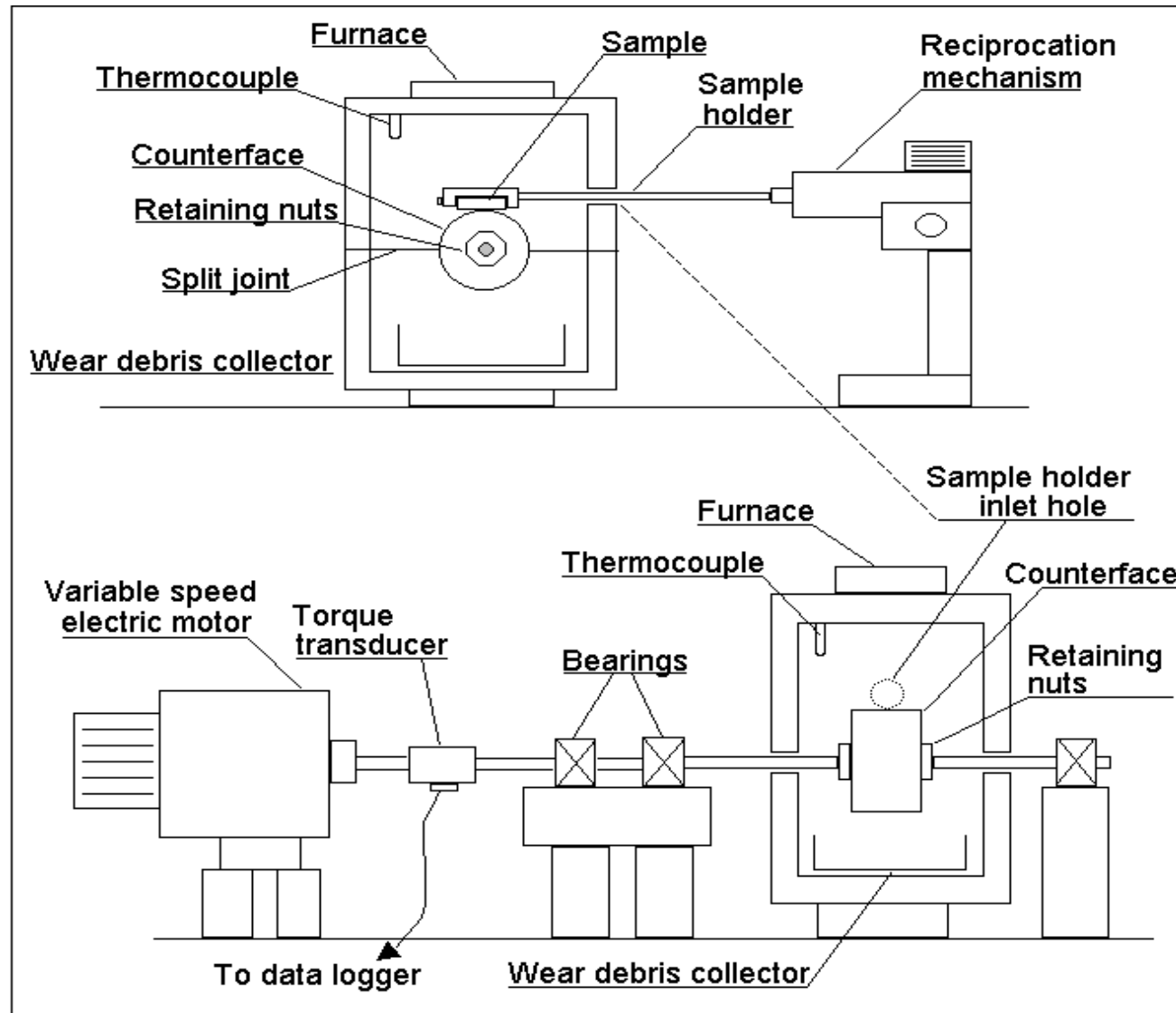
Fig. 1. Reciprocating high temperature block-on-cylinder wear rig, as used in the experimental programme
