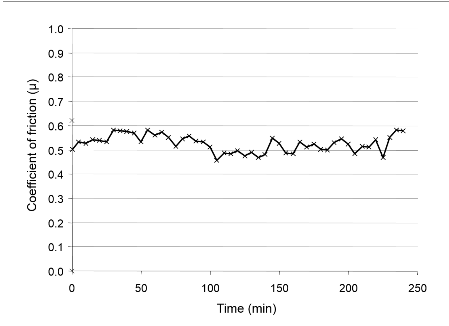
Fig. 3. Coefficient of friction vs. time for Nimonic 80A vs. Stellite 6 at 0.314 \text{ m.s}^{-1} / 750^{\circ}\text{C}
