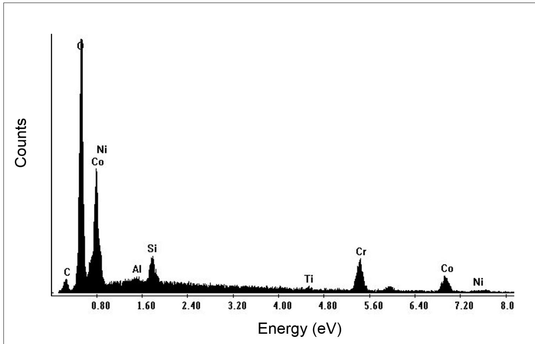
Fig. 4. EDX surface spectrum for Nimonic 80A vs. Stellite 6 at 0.314 \text{ m.s}^{-1} / 750^\circ\text{C}
