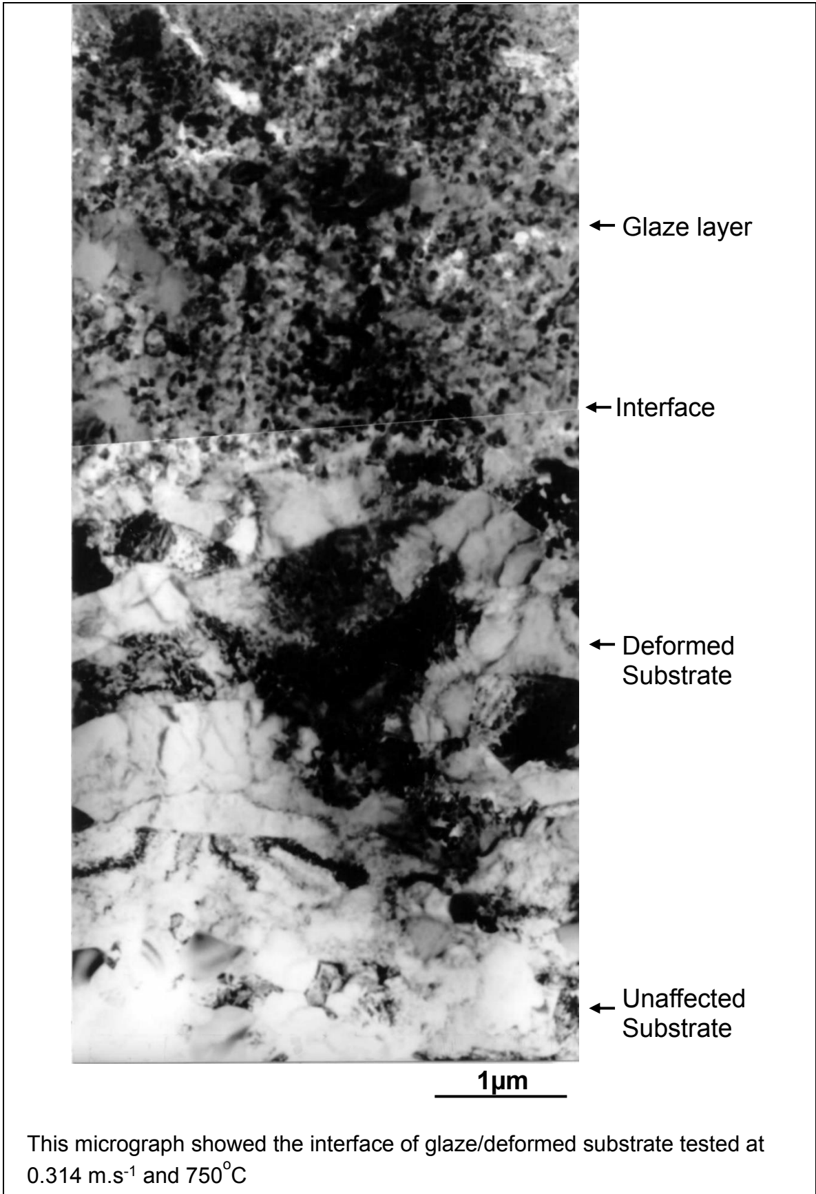
Fig. 8. TEM image showing interface of glaze layer/deformed substrate
