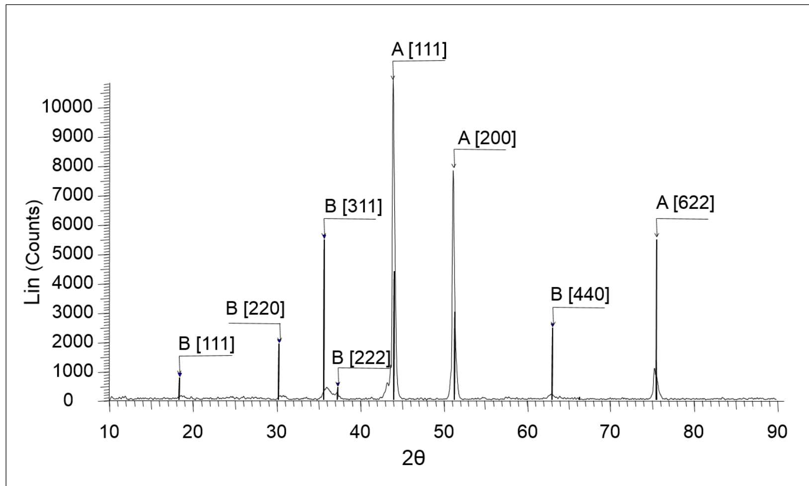
Fig. 5. XRD pattern for Nimonic 80A vs. Stellite 6 at 0.314 \text{ m}\cdot\text{s}^{-1} / 750^\circ\text{C} : (A) \text{Ni}_{2.9}\text{Cr}_{0.7}\text{Fe}_{0.36} ; (B) \text{CoCr}_2\text{O}_4 .
