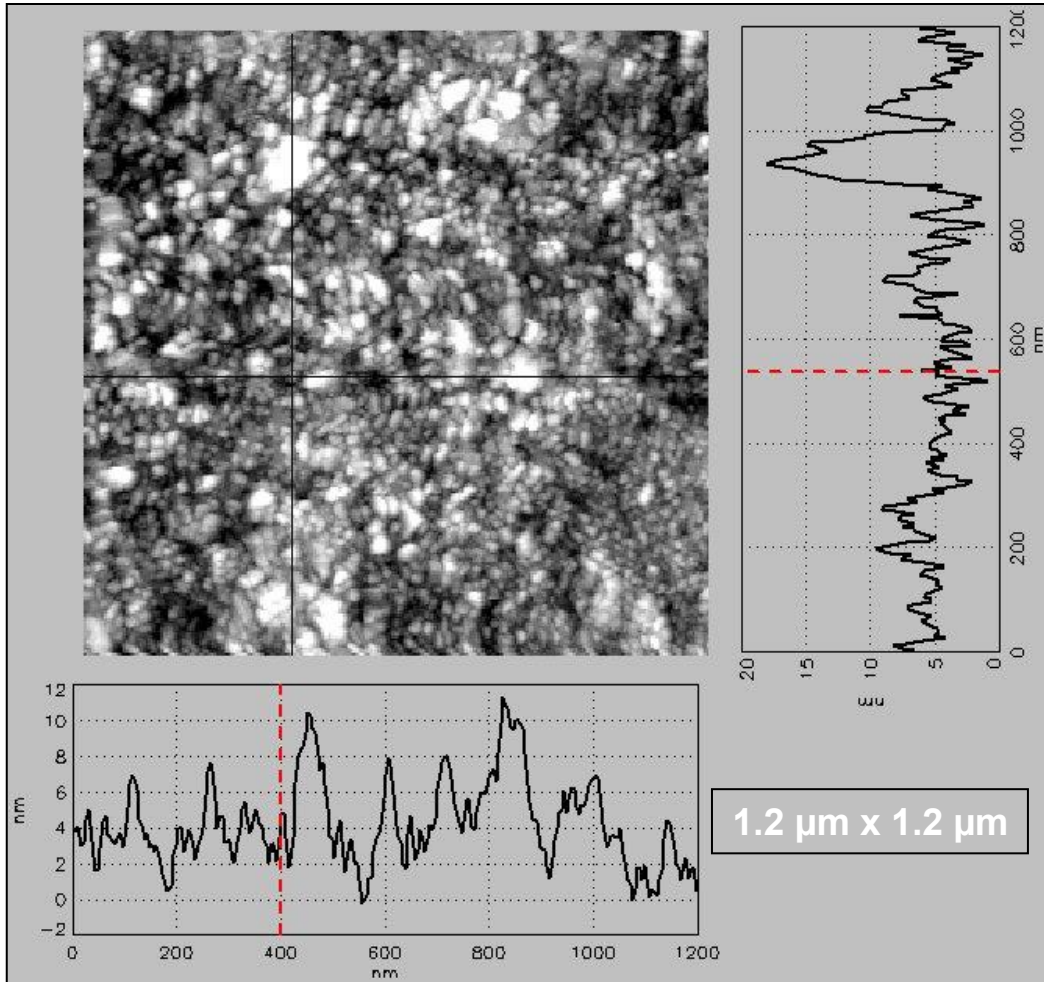
Fig. 9. STM surface line profile results on glaze layer formed on Nimonic 80A at 750°C ( 0.314 \text{ m.s}^{-1} )
