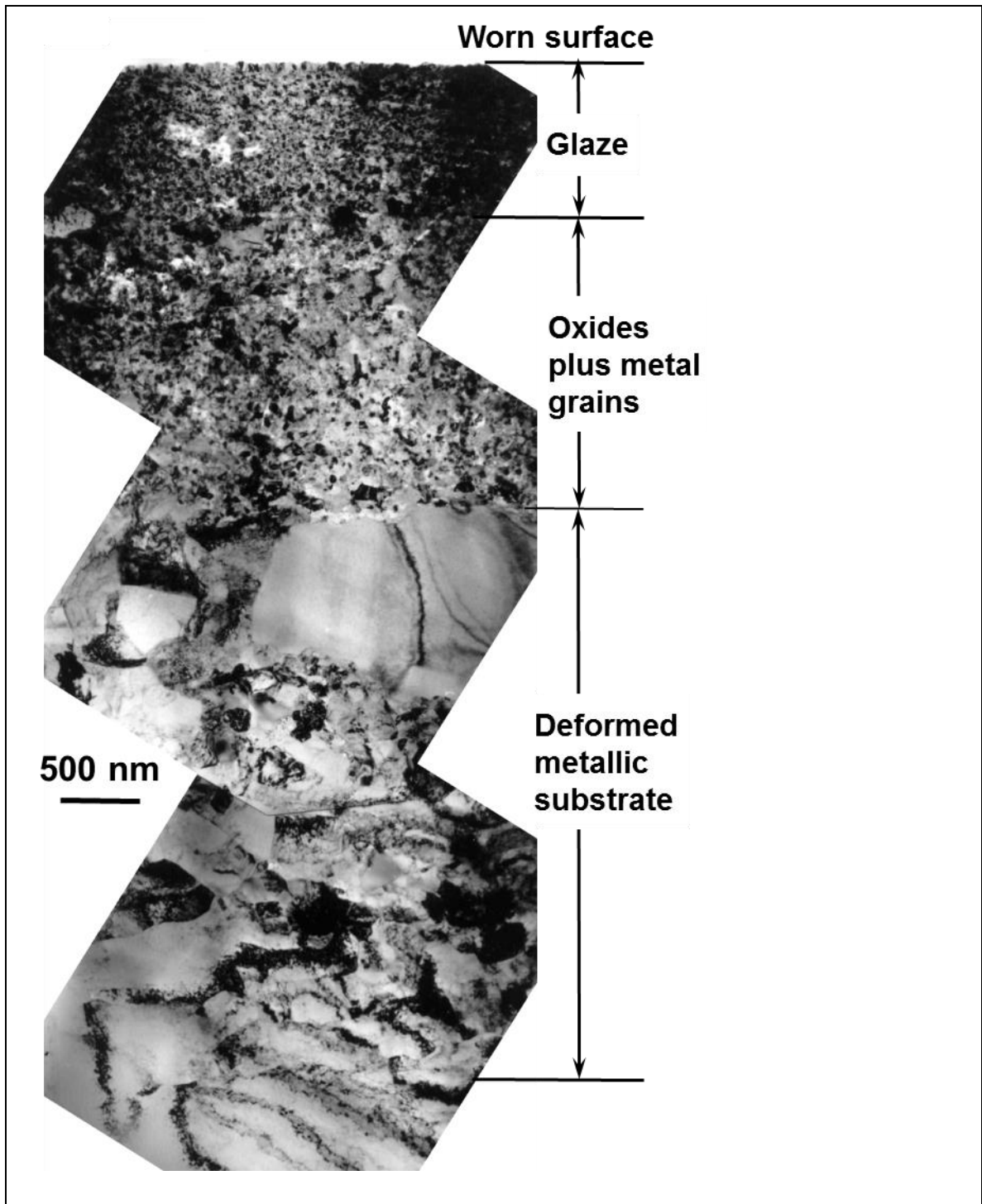
Fig. 6. TEM bright field image: wear-induced polycrystalline glaze layer and deformation of substrate ( 0.314 \text{ m}\cdot\text{s}^{-1} , 750^\circ\text{C} )
