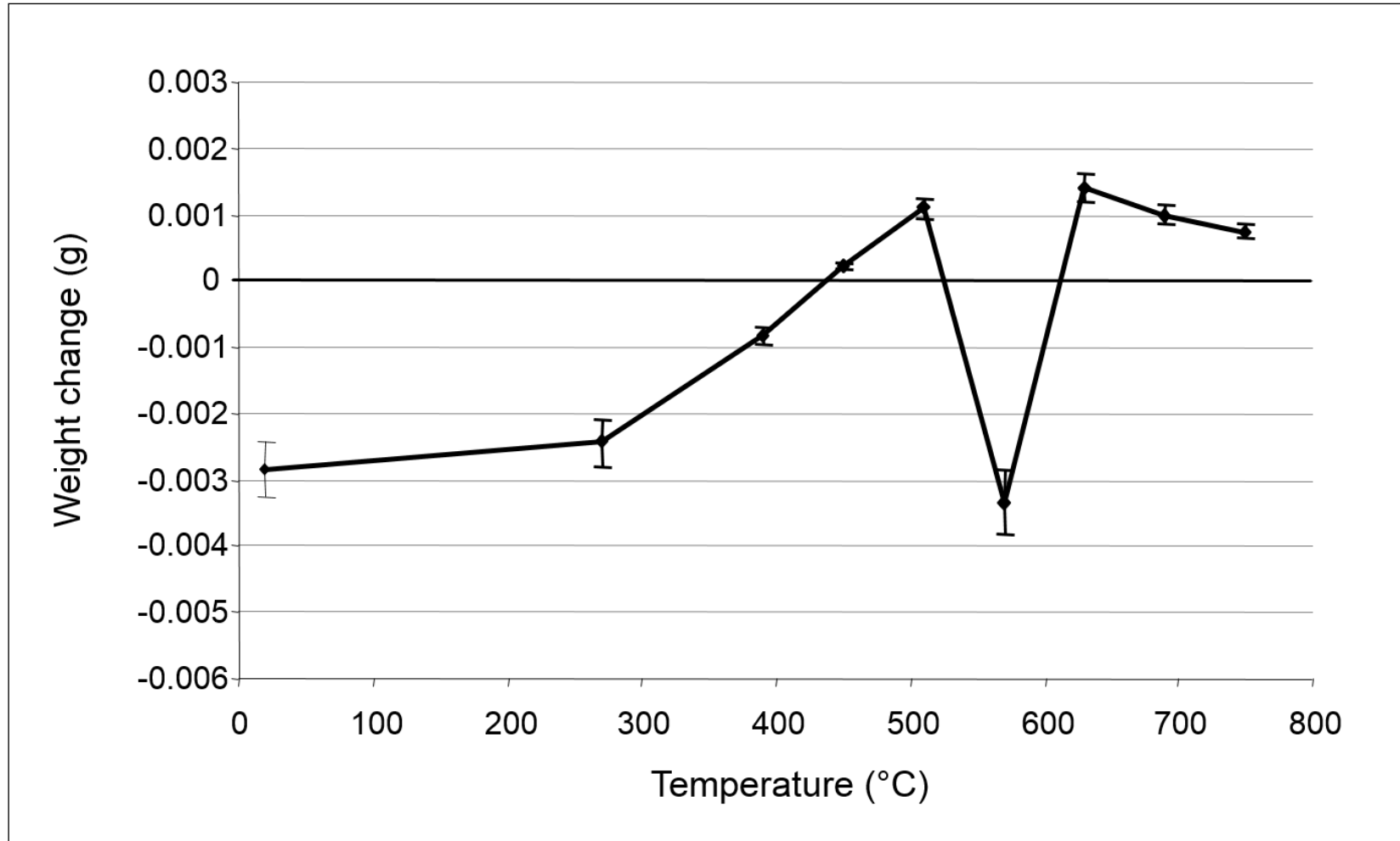
Fig. 2. Weight change vs. temperature for Nimonic 80A against Stellite 6 at 0.314 m.s -1 / 750°C
