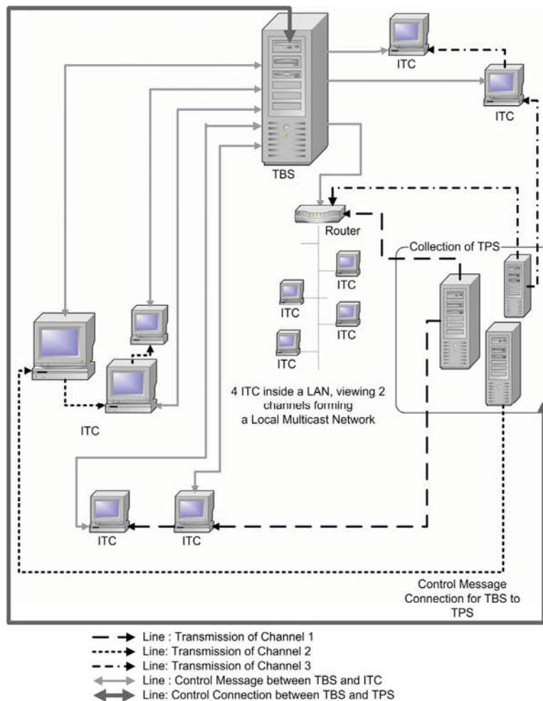
Fig. 2: Communication setup among TBS, TPS and ITC
