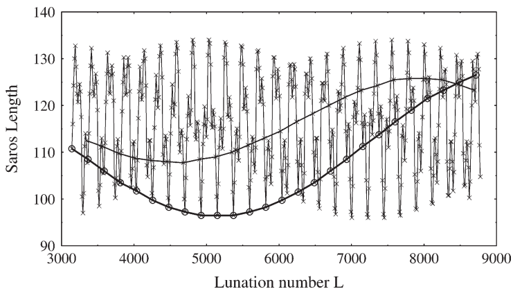
Fig. 6. The Saros length given for all 'odd' eclipse possibilities (EPs) during the first 25 cycles of the Saros cycle (SC) scheme, i.e. from 6 February 747 BC (= SC 1) until 8 June 297 BC (= SC 26), is drawn with a thin line. On the top of this curve, the first EPs for all 25 columns of the SC scheme are marked by a circle and connected by the thick line. The second thick line shows the Saros length from EP 35, i.e. the EPs at intervals of a Saros stemming from the EPs in line 35 of the scheme.
