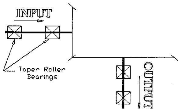
SINGLE STAGE BEVEL GEAR-BOX
