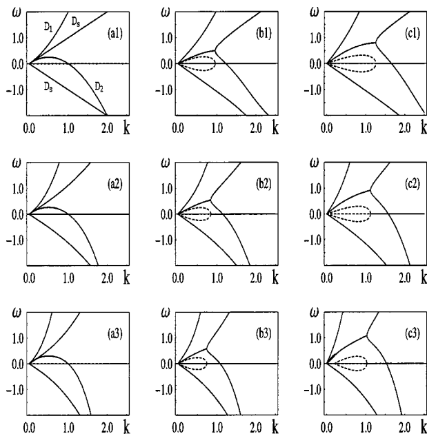
FIG. 4. Real (solid lines) and imaginary (dashed lines) components of the frequency \omega as a function of k for uncoupled [frames (a1), (a2), and (a3)] and coupled cases [frames (b1) to (c3)]. From top to bottom, H=0 , H=0.5 , and H=0.9 , respectively. From left to right, E_0=0 , E_0=0.5 , and E_0=0.5 . For the first and second columns k_0=0.5 ; for the third column, k_0=0.75 . In the first frame, D_i ( i=s, 1, 2 ) indicate the various branches of Eq. (44). A similar labeling applies to all the frames.
