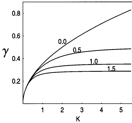
FIG. 1. Growth rate of the decay instability for E_0=0.5 and 0 \leq H \leq 1.5 , as indicated. Notice the quick saturation effect for H > 0 .
