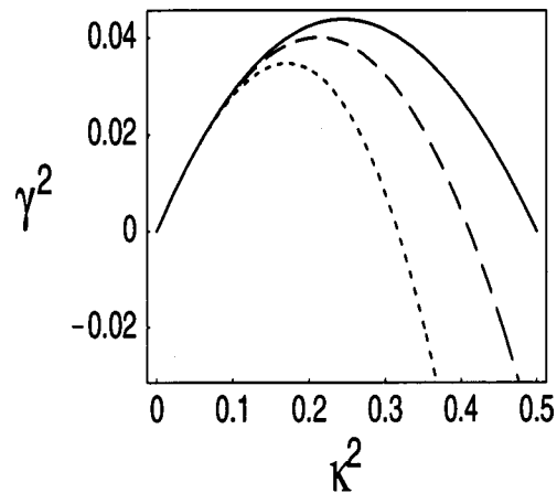
FIG. 2. \gamma^2 as a function of k^2 for the positive root in the dispersion relation (49) for the four-wave instability. We have E_0=0.5 , H=0 (full line), H=0.5 (dashed line), and H=0.9 (dotted line).
