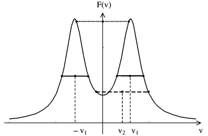
FIG. 2. Semiclassical ( v_0 = \pm v_1 , solid horizontal lines) and purely quantum ( v_0 = \pm v_2 , dashed horizontal line) solutions of Eq. (8) for a symmetrical two-stream equilibrium. Also note that v_0 = 0 (dotted line) is always a solution. Units are conveniently rescaled.
