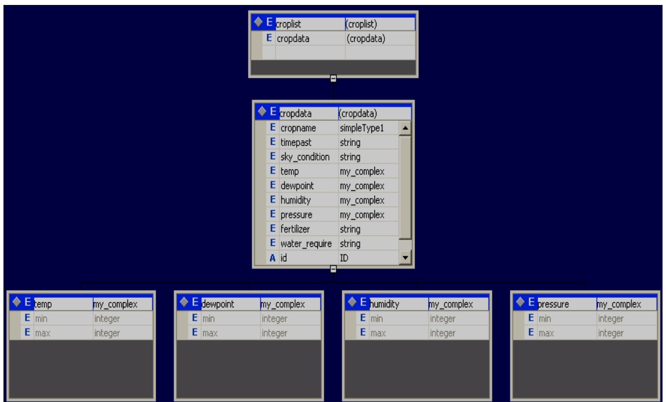
Fig 4: Schema of the AgriExpert system deployed locally
