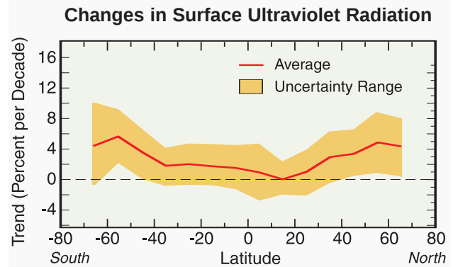
Figure Q17-1. Changes in surface UV radiation. Ultraviolet (UV) radiation at Earth's surface has increased over much of the globe since 1979. Also known as "erythema radiation," sunburning UV is harmful to humans and other life forms. The increases shown here for 1979-1998 are estimated from observed decreases in ozone and the relationship between ozone and surface UV established at some surface locations. The estimates are based on the assumption that all other factors that influence the amount of UV radiation reaching the Earth's surface, such as aerosol abundances and cloudiness, are unchanged. The estimated changes in ultraviolet radiation in the tropics are the smallest because observed ozone changes are the smallest there.
