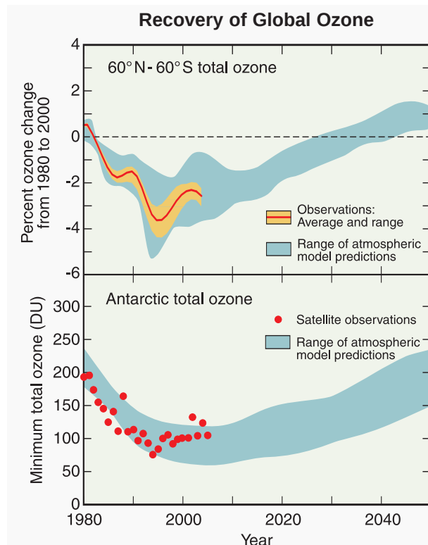
Figure Q20-1. Global ozone recovery predictions. Observed values of midlatitude total ozone (top panel) and September-October minimum total ozone values, over Antarctica (bottom panel) have decreased beginning in the early 1980s. As halogen source gas emissions decrease in the 21 st century, ozone values are expected to recover by increasing toward pre-1980 values. Atmospheric computer models that account for changes in halogen gases and other atmospheric parameters are used to predict how ozone amounts will increase. These model results show that full recovery is expected in midlatitudes by 2050, or perhaps earlier. Recovery in the Antarctic will occur somewhat later. The range of model projections comes from the use of several different models of the future atmosphere.
