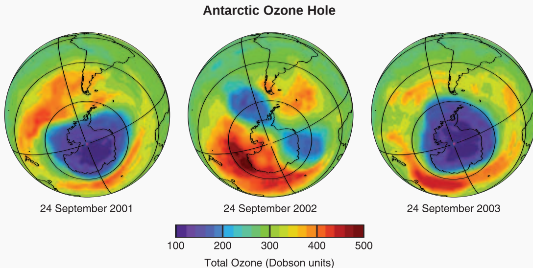
Figure Q11-Box. Anomalous 2002 ozone hole. Views from space of the Antarctic ozone hole as observed on 24 September in each of three consecutive years. The hole split and elongated in 2002, reducing the total depletion of ozone observed that year in comparison with 2001 and 2003. The anomalous depletion in 2002 is attributable to an early warming of the polar stratosphere caused by air disturbances originating in midlatitudes, rather than to large changes in the amounts of reactive chlorine and bromine in the Antarctic stratosphere.
