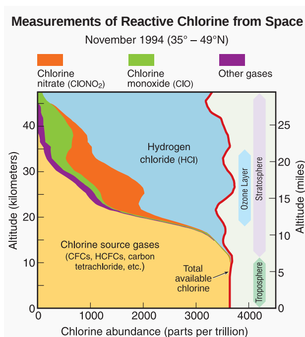
Figure Q8-2. Reactive chlorine gas observations.
