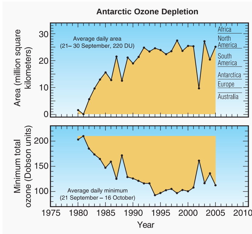
Figure Q11-2. Antarctic ozone hole features. Values are shown for key parameters of the Antarctic ozone hole: the area enclosed by the 220-DU total ozone contour and the minimum total ozone amount, as determined from space-based observations. The values are averaged for each year near the peak of ozone depletion, as defined by the dates shown in each panel. The ozone hole areas are contrasted to the areas of continents in the upper panel. The intensity of ozone depletion gradually increased beginning in 1980. In the 1990s, the depletion reached fairly steady values, except for the anomalously low depletion in 2002 (see Figure Q11-box). The intensity of Antarctic ozone depletion will decrease as part of the ozone recovery process (see Q19 and Q20).
