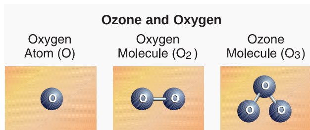
Figure Q1-1. Ozone and oxygen. A molecule of ozone ( O_3 ) contains three oxygen (O) atoms bound together. Oxygen molecules ( O_2 ), which constitute 21% of Earth’s atmosphere, contain two oxygen atoms bound together.
