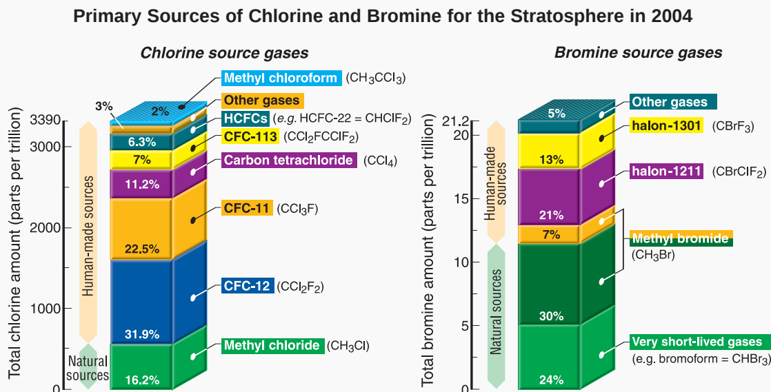
Figure Q7-1. Stratospheric source gases. A variety of gases transport chlorine and bromine into the stratosphere. These gases, called halogen source gases, are emitted from natural sources and by human activities. These partitioned columns show how the principal chlorine and bromine source gases contribute to the respective total amounts of chlorine and bromine as measured in 2004. Note the large difference in the vertical scales: total chlorine in the stratosphere is 160 times more abundant than total bromine. For chlorine, human activities account for most that reaches the stratosphere. The CFCs are the most abundant of the chlorine-containing gases released in human activities. Methyl chloride is the most important natural source of chlorine. HCFCs, which are substitute gases for CFCs and also are regulated under the Montreal Protocol, are a small but growing fraction of chlorine-containing gases. The “Other gases” category includes minor CFCs and short-lived gases. For bromine that reaches the stratosphere, halons and methyl bromide are the largest sources. Both gases are released in human activities. Methyl bromide has an additional natural source. Natural sources are a larger fraction of total bromine than of total chlorine. (The unit “parts per trillion” is used here as a measure of the relative abundance of a gas in air: 1 part per trillion indicates the presence of one molecule of a gas per trillion other air molecules.)
