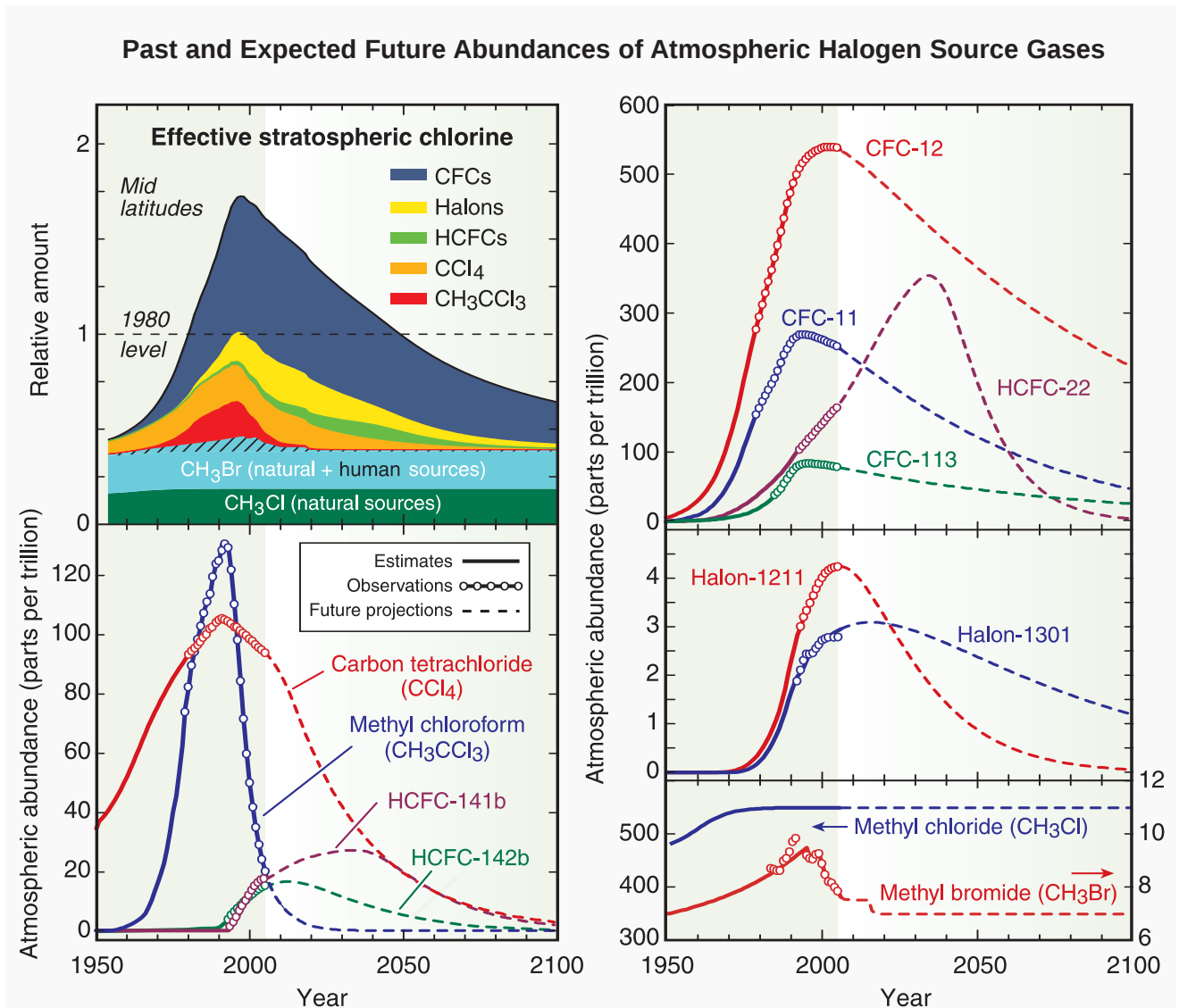
Figure Q16-1. Halogen source gas changes. The rise in effective stratospheric chlorine values in the 20 th century has slowed and reversed in the last decade (top left panel). Effective stratospheric chlorine values are a measure of the potential for ozone depletion in the stratosphere, obtained by summing over adjusted amounts of all chlorine and bromine gases. Effective stratospheric chlorine levels as shown here for midlatitudes will return to 1980 values around 2050. The return to 1980 values will occur around 2065 in polar regions. In 1980, ozone was not significantly depleted by the chlorine and bromine then present in the stratosphere. A decrease in effective stratospheric chlorine abundance follows reductions in emissions of individual halogen source gases. Overall emissions and atmospheric concentrations have decreased and will continue to decrease given international compliance with the Montreal Protocol provisions (see Q15). The changes in the atmospheric abundance of individual gases at Earth's surface shown in the panels were obtained using a combination of direct atmospheric measurements, estimates of historical abundance, and future projections of abundance. The past increases of CFCs, along with those of CCl 4 and CH 3 CCl 3 , have slowed significantly and most have reversed in the last decade. HCFCs, which are used as CFC substitutes, will continue to increase in the coming decades. Some halon abundances will also continue to grow in the future while current halon reserves are depleted. Smaller relative decreases are expected for CH 3 Br in response to production and use restrictions because it has substantial natural sources. CH 3 Cl has large natural sources and is not regulated under the Montreal Protocol. (See Figure Q7-1 for chemical names and formulas. The unit "parts per trillion" is defined in the caption of Figure Q7-1.)
