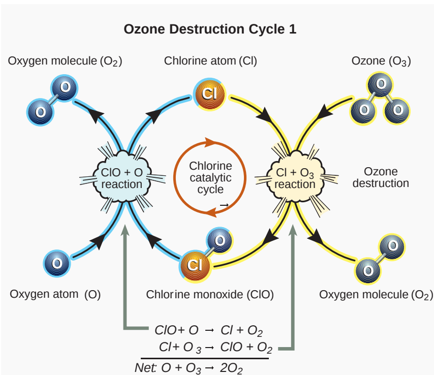
Figure Q9-1. Ozone destruction
