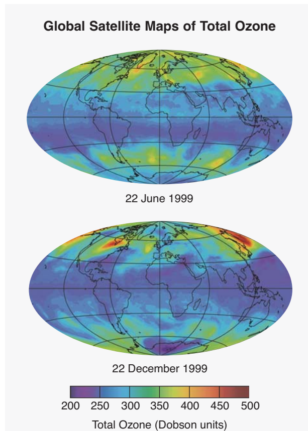
Figure Q4-1. Total ozone. A total ozone value is obtained by measuring all the ozone that resides in the atmosphere over a given location on Earth’s surface. Total ozone values shown here are reported in “Dobson units” as measured by a satellite instrument from space. Total ozone varies with latitude, longitude, and season, with the largest values at high latitudes and the lowest values in tropical regions. Total ozone at most locations varies with time on a daily to seasonal basis as ozone-rich air is moved about the globe by stratospheric winds. Low total ozone values over Antarctica in the 22 December image represent the remainder of the “ozone hole” from the 1999 Antarctic winter/spring season (see Q11).
