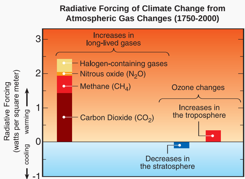
Figure Q18-1. Radiative forcing of climate change from atmospheric gas changes.
