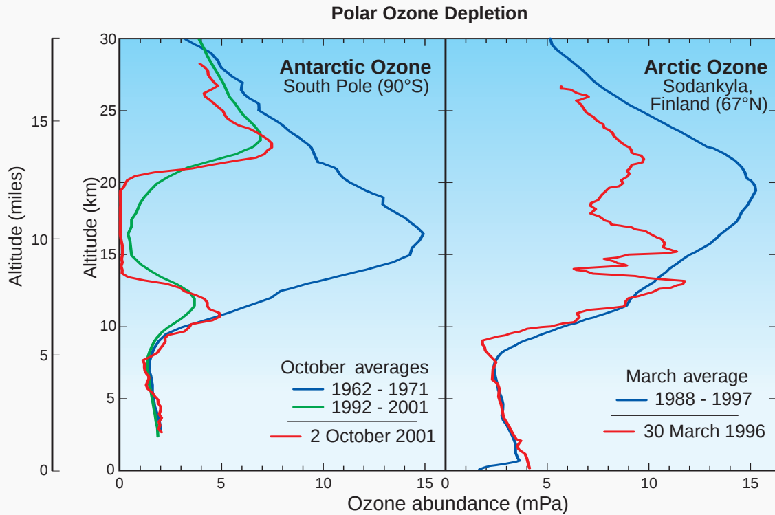
Figure Q11-3. Arctic and Antarctic ozone distribution. The stratospheric ozone layer resides between about 10 and 50 kilometers (6 to 31 miles) above Earth's surface over the globe. Long-term observations of the ozone layer with balloonborne instruments allow the winter Antarctic and Arctic regions to be compared. In the Antarctic at the South Pole, halogen gases have destroyed ozone in the ozone layer beginning in the 1980s. Before that period, the ozone layer was clearly present, as shown here using average ozone values from balloon observations made between 1962 and 1971. In more recent years, as shown here for 2 October 2001, ozone is destroyed completely between 14 and 20 kilometers (8 to 12 miles) in the Antarctic in spring. Average October values in the ozone layer now are reduced by 90% from pre-1980 values. The Arctic ozone layer is still present in spring as shown by the average March profile obtained over Finland between 1988 and 1997. However, March Arctic ozone values in some years are often below normal average values as shown here for 30 March 1996. In such years, winter minimum temperatures are generally below PSC formation temperatures for long periods. Ozone abundances are shown here with the unit "milli-Pascals" (mPa), which is a measure of absolute pressure (100 million mPa = atmospheric sea-level pressure).
