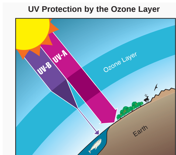
Figure Q3-1. UV-B protection by the ozone layer. The ozone layer resides in the stratosphere and surrounds the entire Earth. UV-B radiation (280- to 315-nanometer (nm) wavelength) from the Sun is partially absorbed in this layer. As a result, the amount of UV-B reaching Earth's surface is greatly reduced. UV-A (315- to 400-nm wavelength) and other solar radiation are not strongly absorbed by the ozone layer. Human exposure to UV-B increases the risk of skin cancer, cataracts, and a suppressed immune system. UV-B exposure can also damage terrestrial plant life, single-cell organisms, and aquatic ecosystems.
