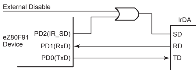
Figure 15. IrDA Hardware Connections
