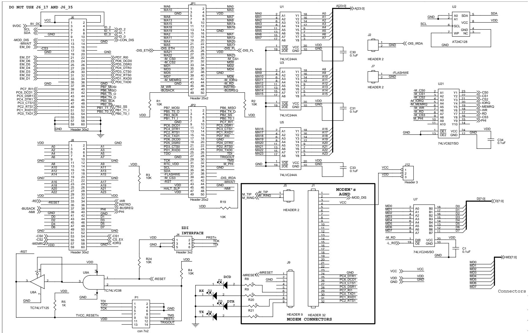
Figure 18. eZ80F91 Development Platform Schematic Diagram, #1 of 5
