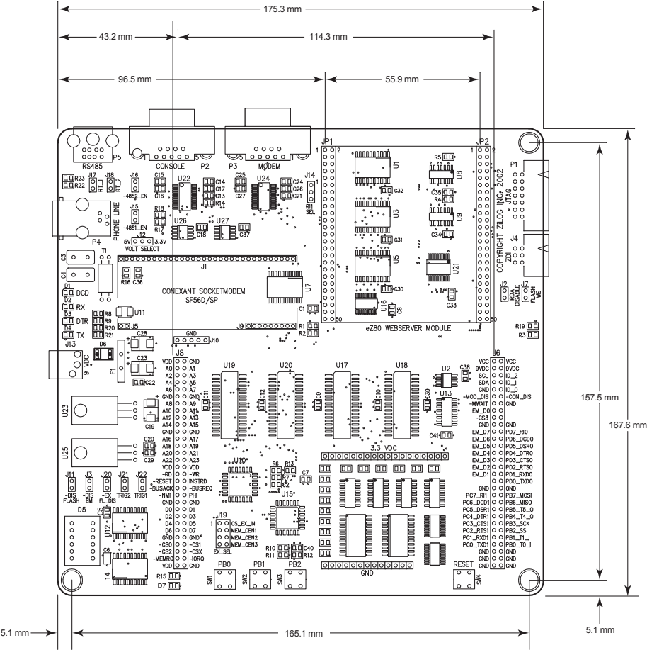
Figure 5. Physical Dimensions of the eZ80 ® Development Kit
