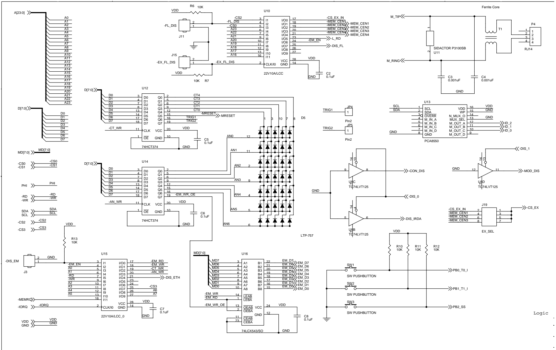
Figure 19. eZ80F91 Development Platform Schematic Diagram, #2 of 5
