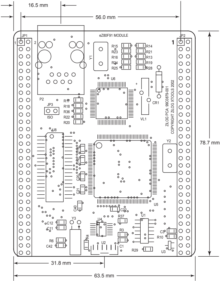
Figure 12. Physical Dimensions of the eZ80F91 Module
