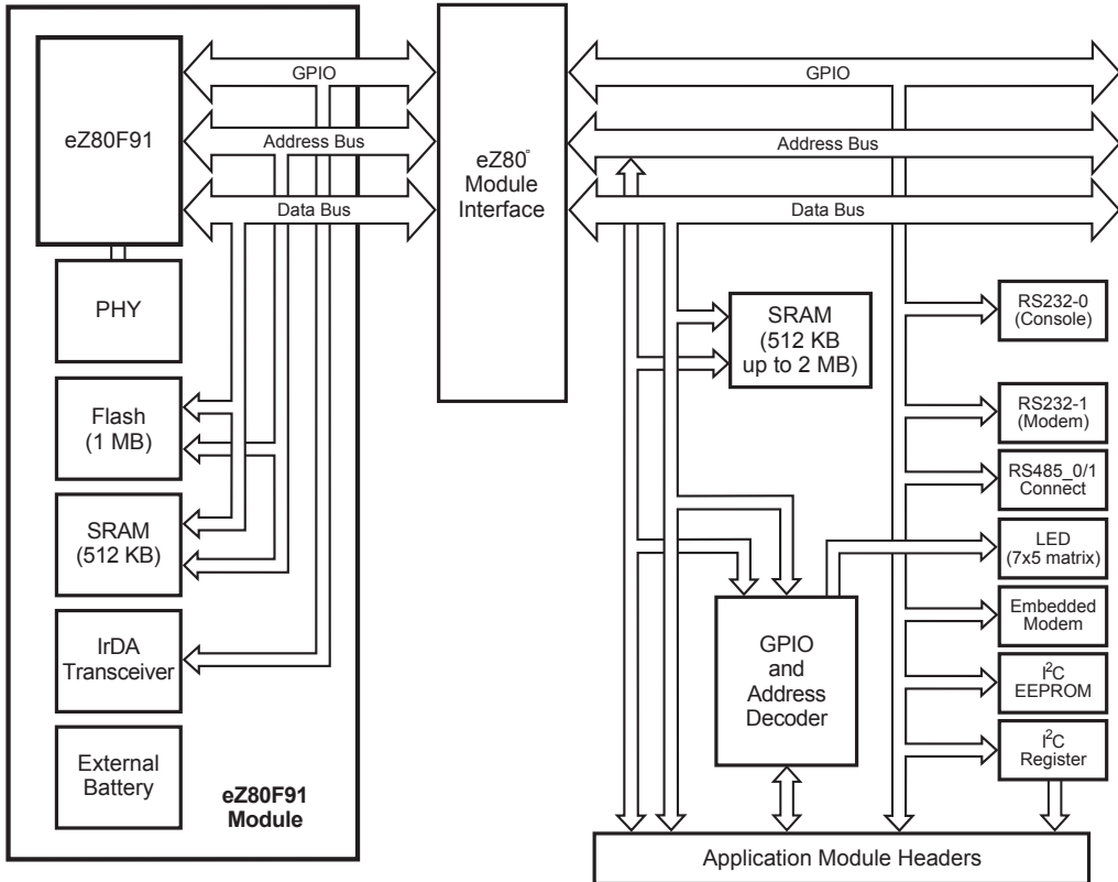
Figure 1. eZ80 ® Development Kit Block Diagram with eZ80F91 Module
