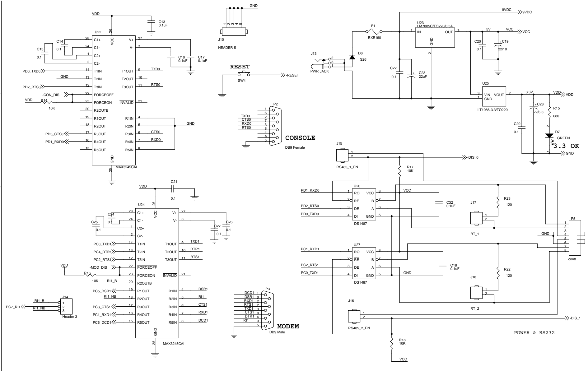
Figure 21. eZ80F91 Development Platform Schematic Diagram, #4 of 5
