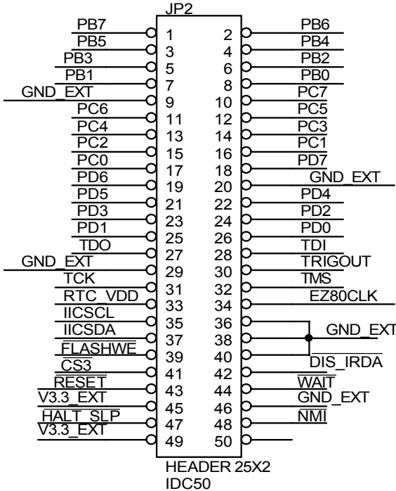
Figure 7. eZ80 ® Development Kit I/O Connector Pin Configuration—JP2
