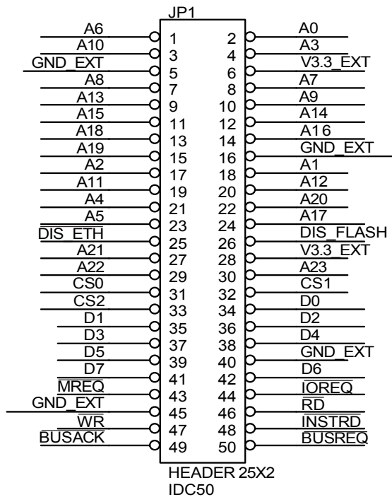
Figure 6. eZ80 ® Development Kit Peripheral Bus Connector Pin Configuration—JP1
