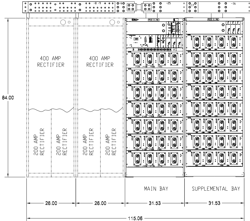
TYPICAL PEC 153M LAYOUT
