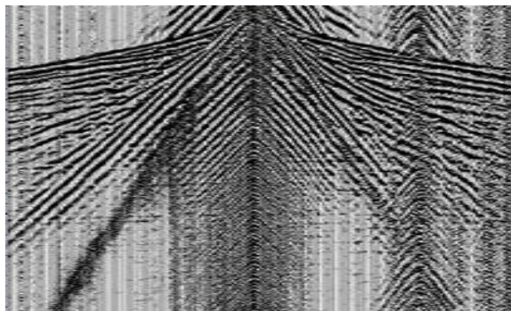
Figure 1: Raw single-sensor cross-spread record.
