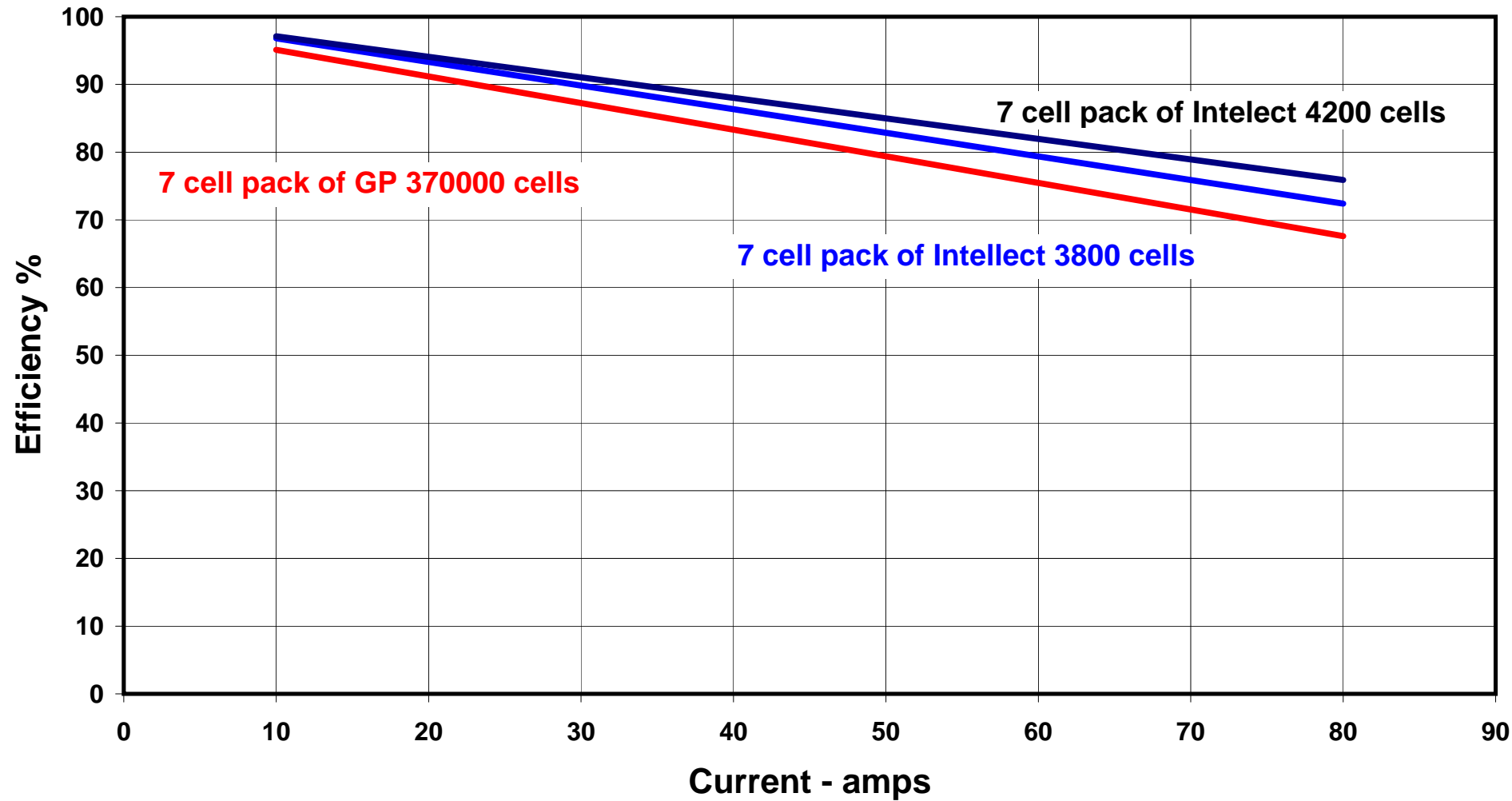
Graph 4 - Battery Efficiency curves - sub C packs
