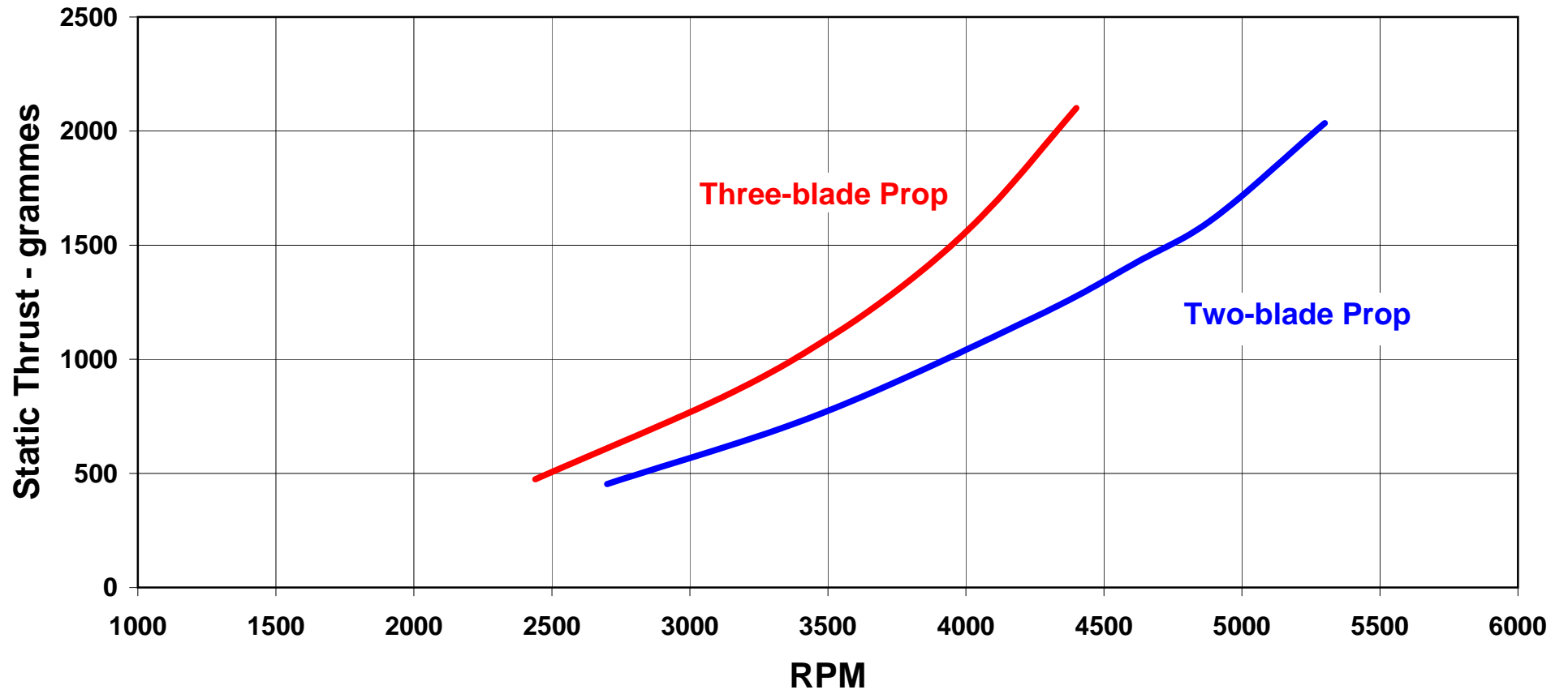
Graph 5 - Propeller Calibration - Aeronaut Cam Folder 15" x 10"
