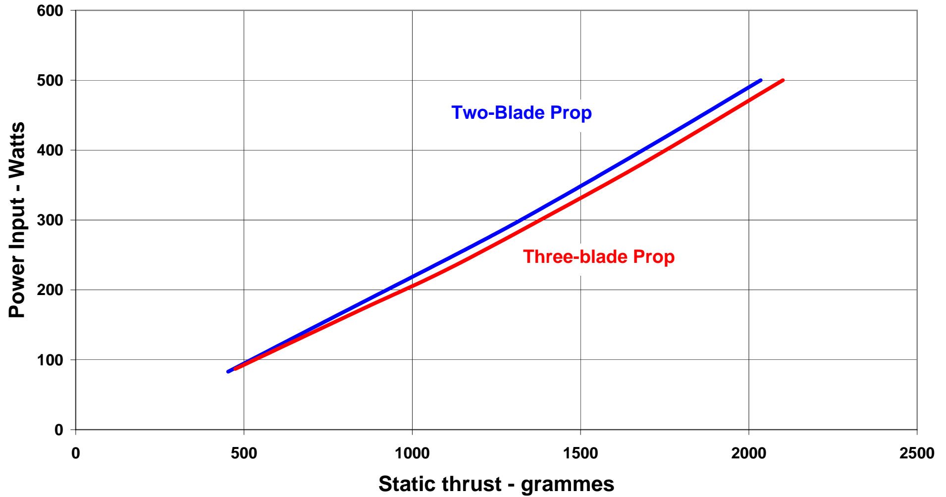
Graph 7 - Power V Static Thrust
