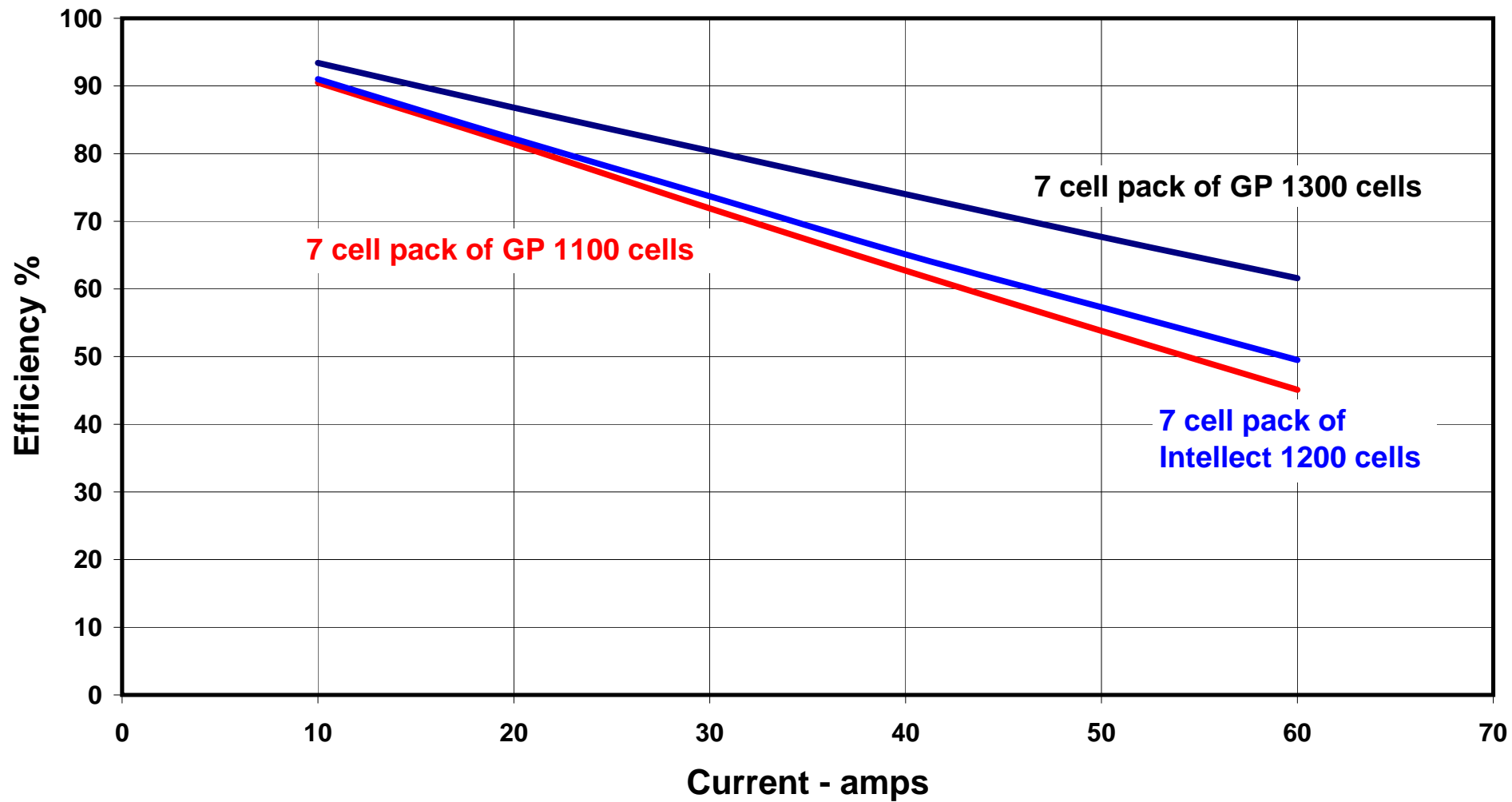
Graph 2 - Battery Efficiency curves
