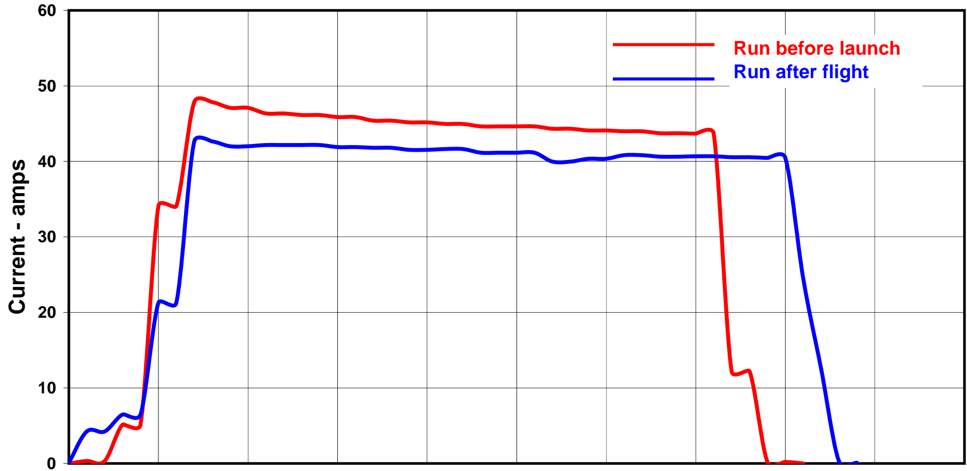
Graph 3 - Big Swift Static Current.
