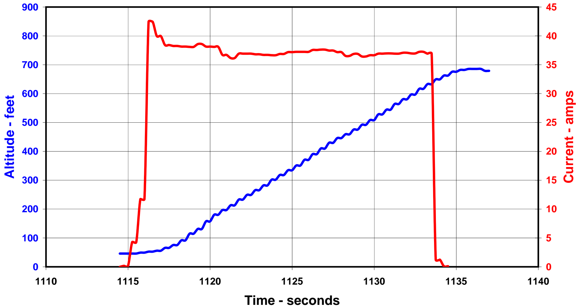
Graph 7 - Big Swift Max Climb J
