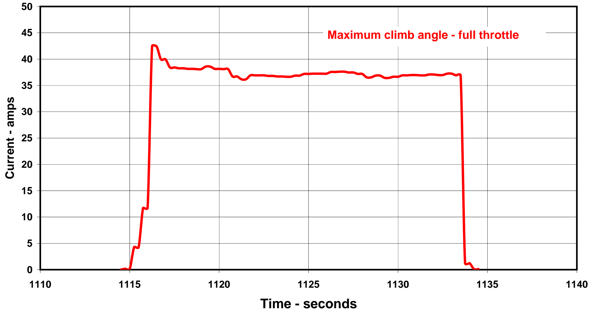
Graph 6 - Big Swift Current V Time (J).
