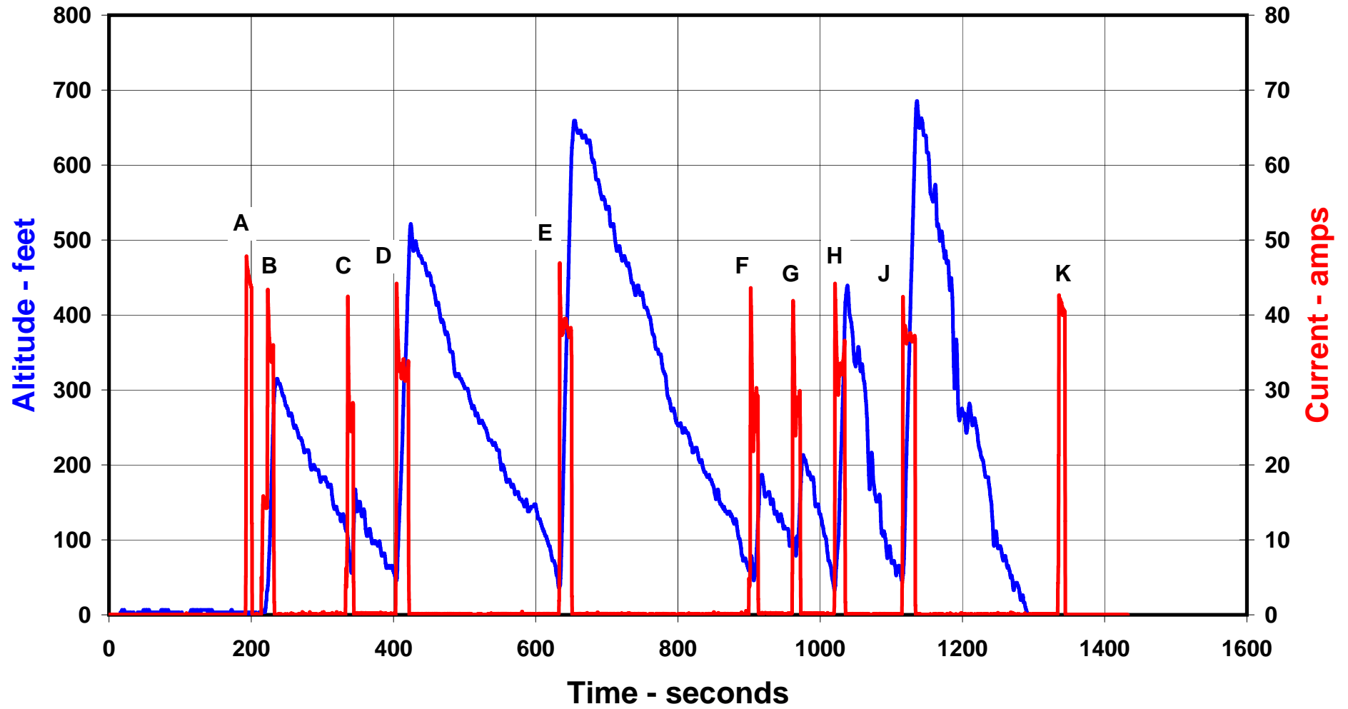
Graph 2 - Big Swift Altitude and Current Draw.
