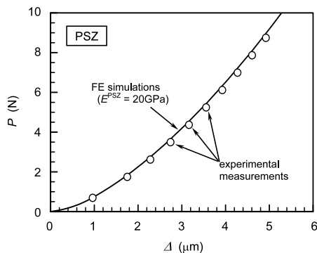
Fig. 5. Simulated load–displacement relation of PSZ with E^{\text{PSZ}} = 20 GPa. The experimental record at selected load levels are shown with circles.
