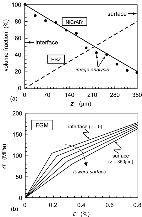
Fig. 11. FGM properties determined from the inverse analysis. (a) Through-thickness variations of PSZ and NiCrAlY volume fractions. (b) Stress–strain relations along different depths of FGM coating.
