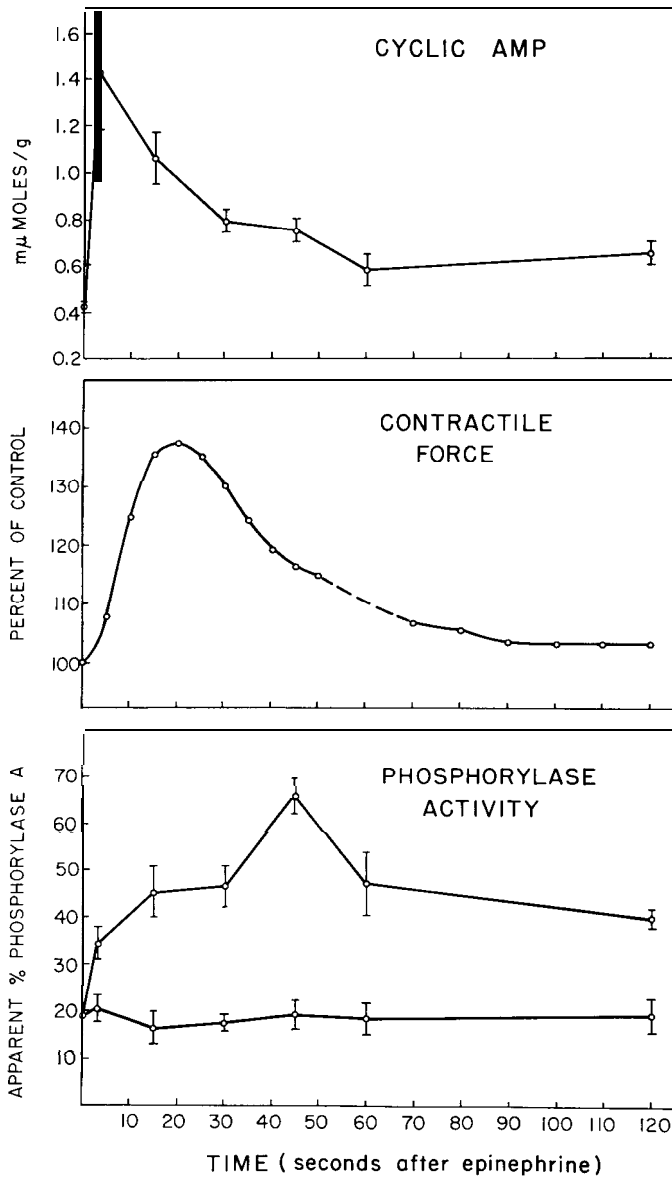
Fig. 6. Effect of a single dose of epinephrine on cyclic AMP - contractile force, and phosphorylase activity in the isolated perfused working rat heart. Hearts were frozen at different times after injection of epinephrine. Lower curve in bottom panel shows lack of response to injected saline. From (28).
