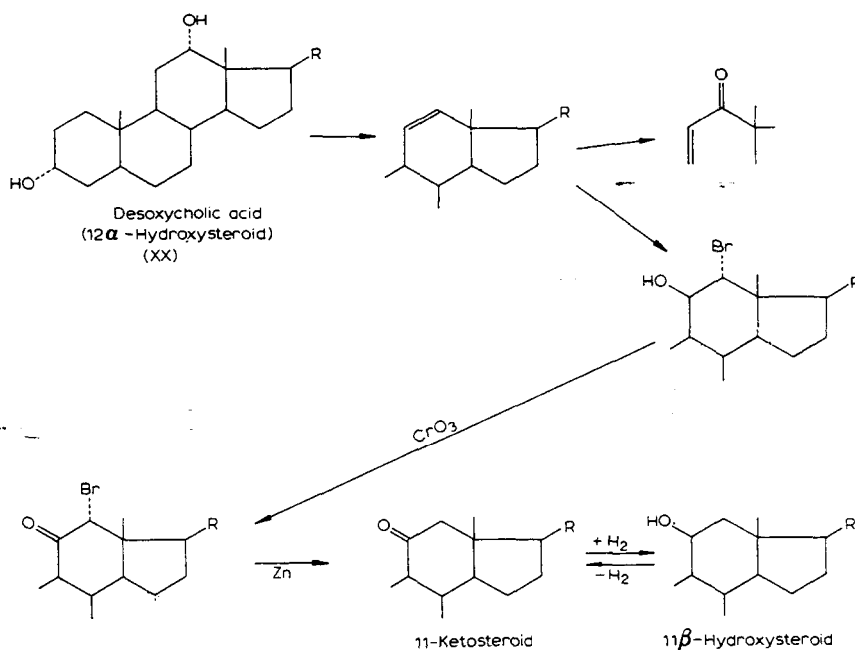
Scheme 5. Introduction of hydroxyl or ketone group in 11 position.
