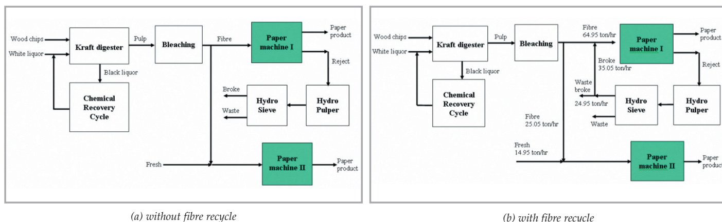
Figure 4: A papermaking process
