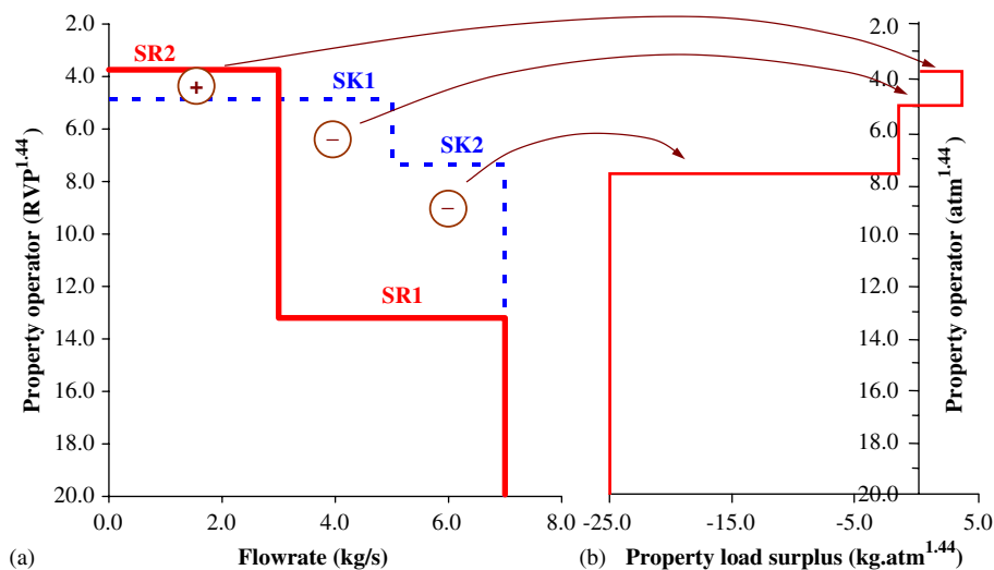
Fig. 4. Construction of a property surplus diagram: (a) sink and source composite plots; (b) property surplus diagram.
