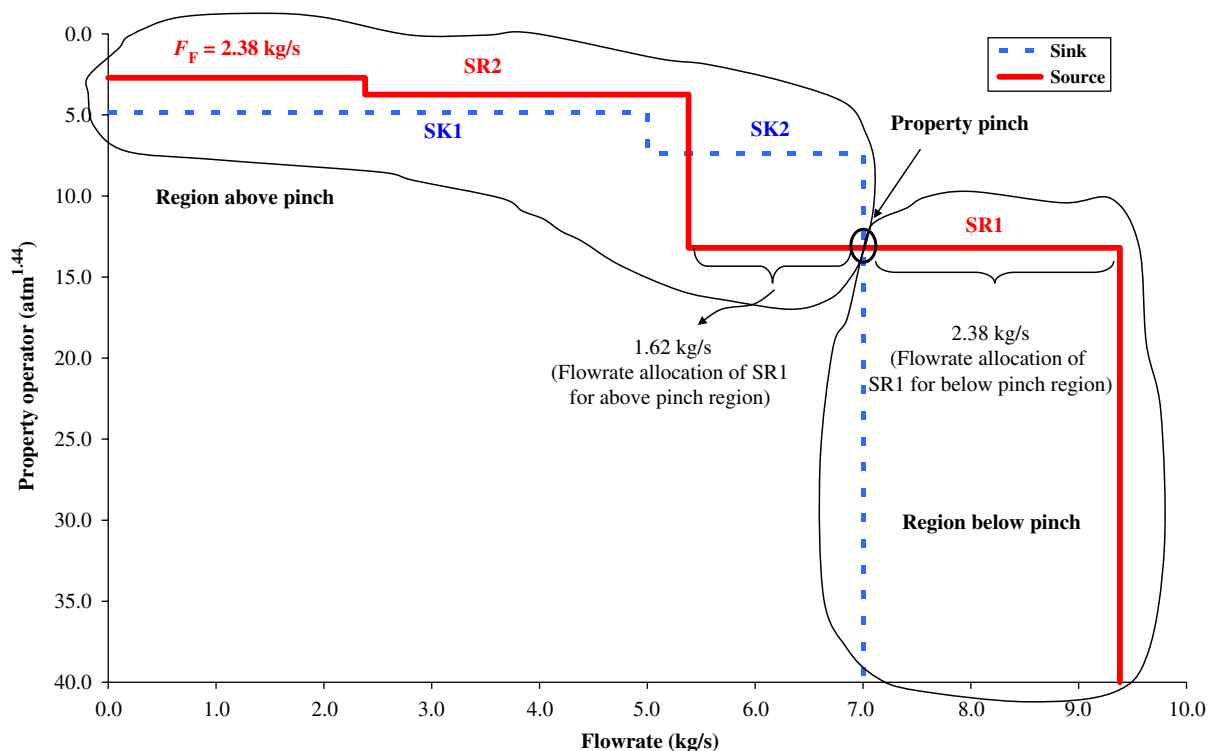
Fig. 10. A feasible property surplus diagram for Example 1.
