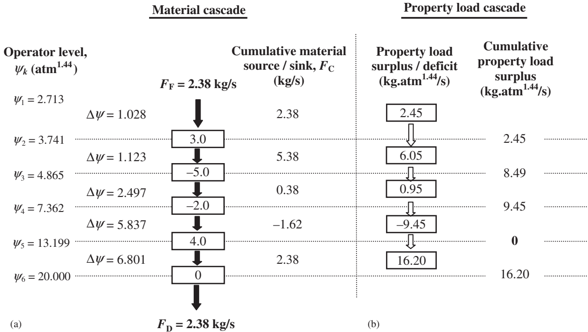
Fig. 8. A feasible material cascade for Example 1.
