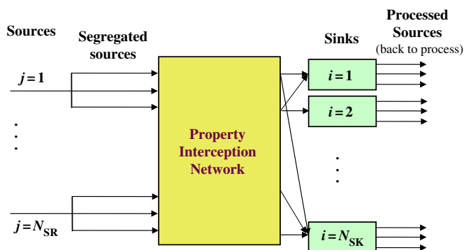
Fig. 1. Source-sink representation for a property-based material reuse network.
