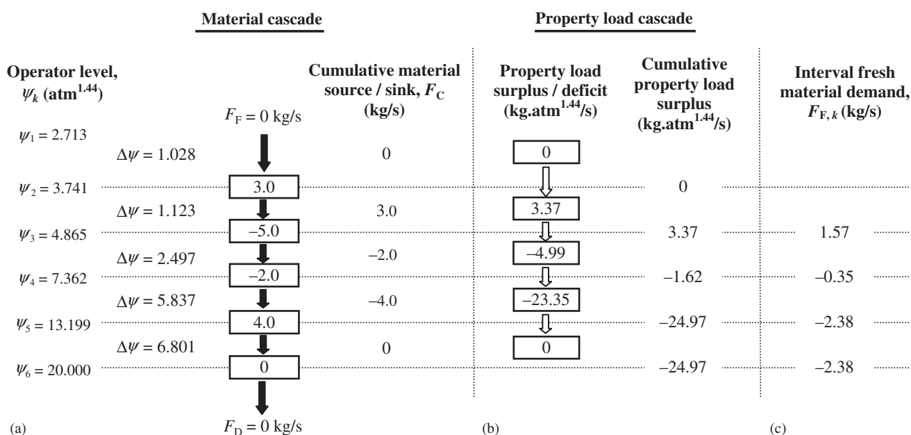
Fig. 6. (a) Material cascade diagram with an assumed fresh solvent flowrate of 0 kg/s; (b) pure property load cascade is used to check the feasibility of the property network; (c) determining interval material flowrates at each purity interval k .
