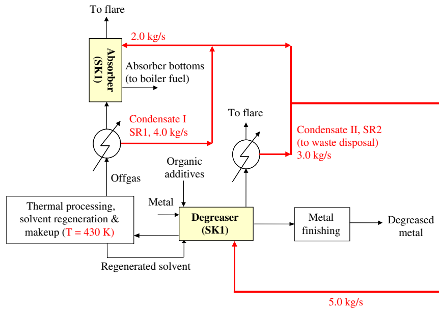
Fig. 13. Network design for metal degreasing process after process modification.
