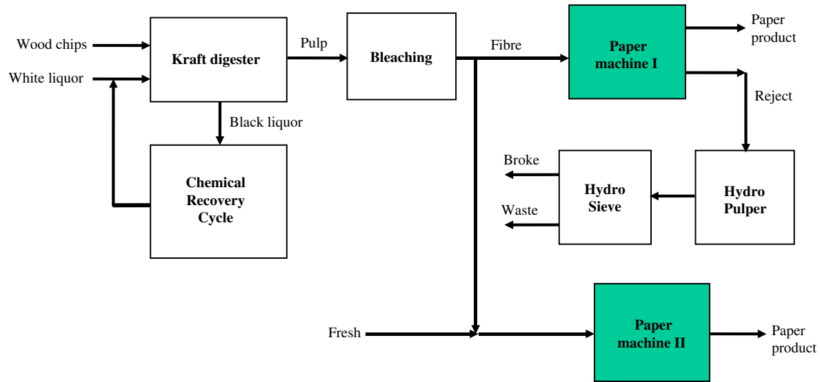
Fig. 14. A papermaking process (Kazantzi and El-Halwagi, 2005).
