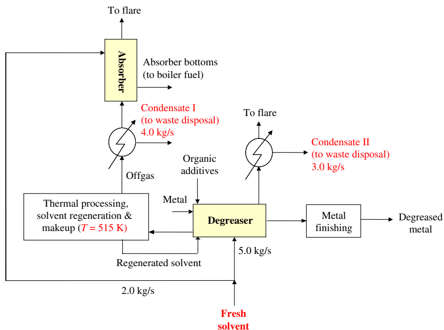
Fig. 2. Example 1: A metal degreasing process (Kazantzi and El-Halwagi, 2005).
