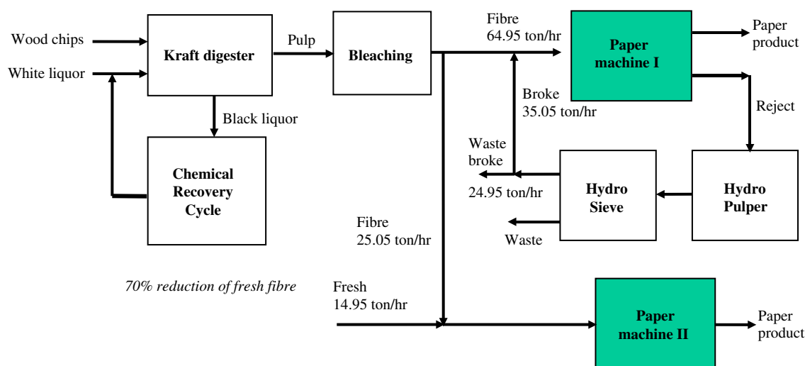
Fig. 15. Final configuration of the papermaking process.
