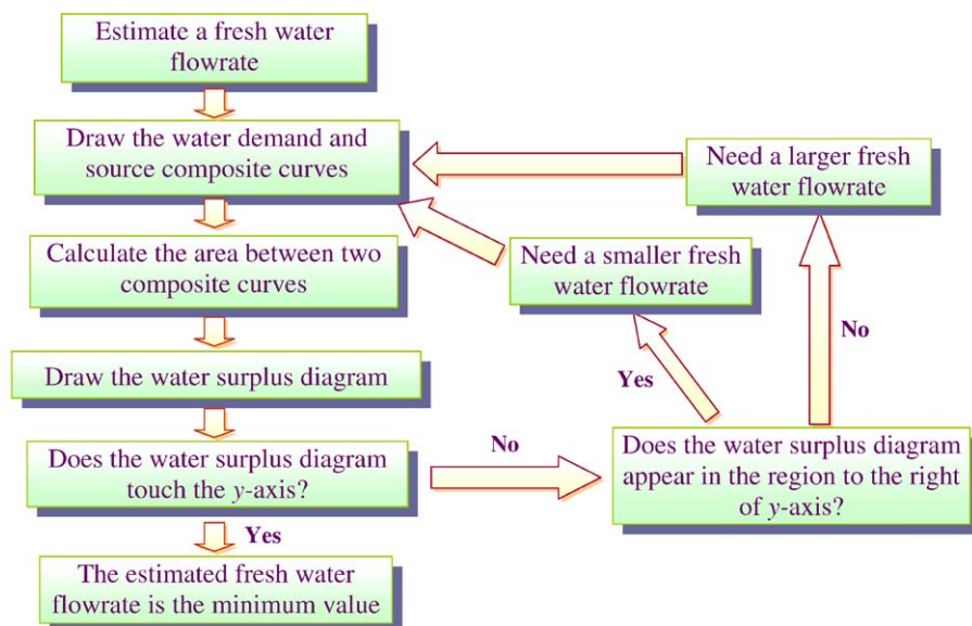
Fig. 5. The tedious iterative steps for constructing a water surplus diagram (Manan et al., 2004).
