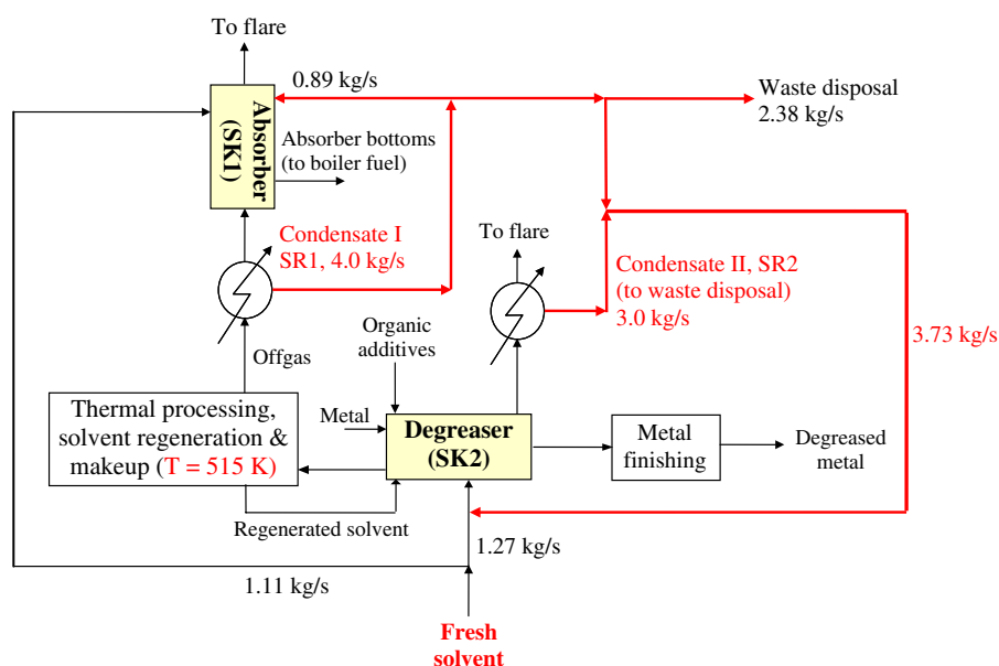
Fig. 12. Network design for degreaser plant to achieve MRR objective (before process modification).
