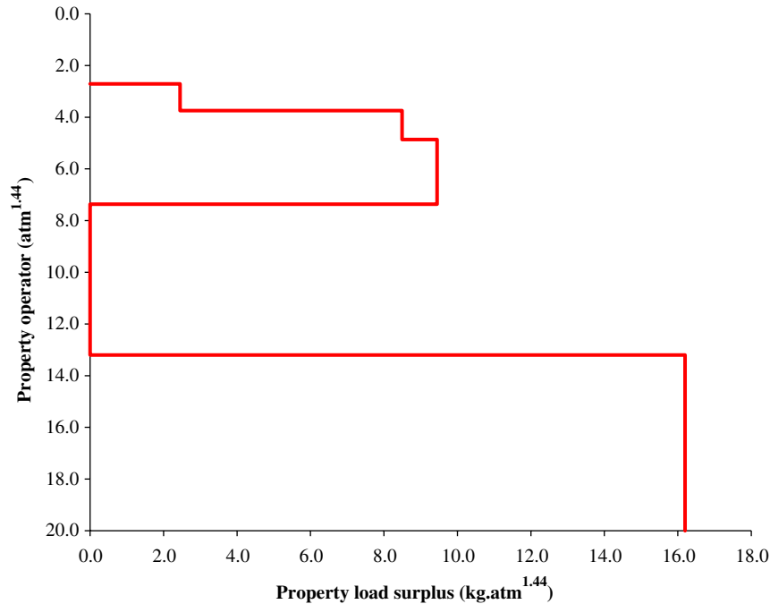
Fig. 9. A feasible property surplus diagram for Example 1.
