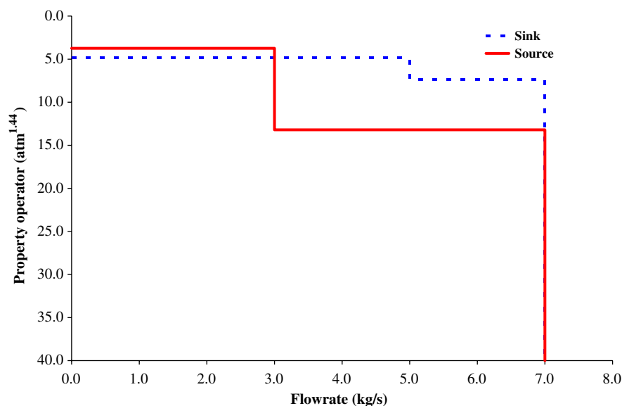
Fig. 3. Sink and source composite plots for Example 1, with the solvent flowrate set to 0 kg/s.
