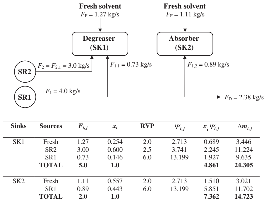
Fig. 11. Network design for Example 1.
