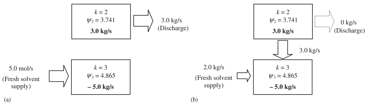
Fig. 7. (a) No solvent cascading; (b) with solvent cascading, discharge is eliminated and fresh solvent intake is reduced.
