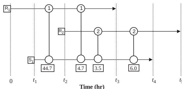
Fig. 3. The OTGD shows the cumulative representation of the entire network throughout the process duration.
