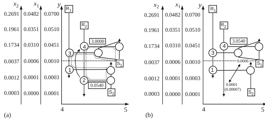
Fig. 14. Mass load loop breaking in the third time interval: (a) mass load shifted from exchanger 2 to exchanger 4; (b) \varepsilon violation occurs at the lean end of exchanger 4 (number in bracket indicates the corresponding target composition of R_2 in S_2 ).
