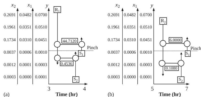
Fig. 6. MEN designs for the (a) second and (b) fourth time intervals.
