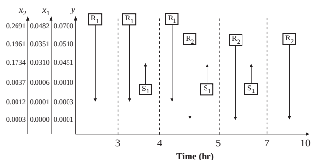
Fig. 4. A TGD showing the process streams for a single-batch COG operation.
