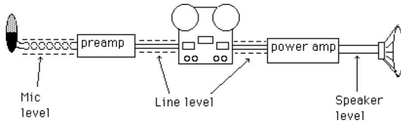
Fig. 1 typical connections
