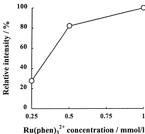
Fig. 2. Effect of the concentration of \text{Ru}(\text{phen})_3^{2+} in 2 mmol/l \text{Ce}(\text{IV}) and 0.08 mol/l \text{H}_2\text{SO}_4 on the emission intensity from 1 \times 10^{-3} mol/l oxalic acid.
