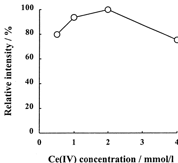
Fig. 3. Effect of the concentration of \text{Ce}(\text{IV}) in 0.08 mol/l \text{H}_2\text{SO}_4 on the emission intensity from 1 \times 10^{-3} mol/l oxalic acid in the presence of 0.25 mmol/l \text{Ru}(\text{phen})_3^{2+} .
