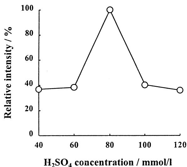
Fig. 4. Effect of the of sulfuric acid in 2 mmol/l \text{Ce}(\text{IV}) on the emission intensity from 1 \times 10^{-3} mol/l oxalic acid in the presence of 0.25 mmol/l \text{Ru}(\text{phen})_3^{2+} .
