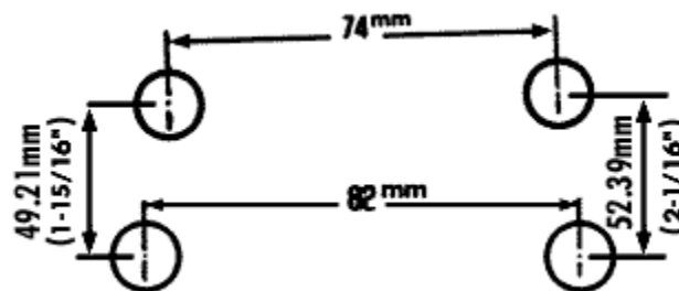
Drilling Dimensions (Do not use as a template)
