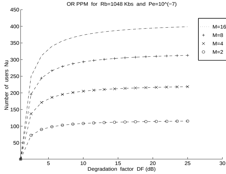
Figure 5.16: The number of users N_u(\text{DF}) for OR PPM signals, calculated for different values of M under perfect power control conditions using R_b = 1048 Kbps, \text{UBP}_b^{\text{OR}}(1) \simeq 10^{-7} and set 1 of parameters in table 5.1.
