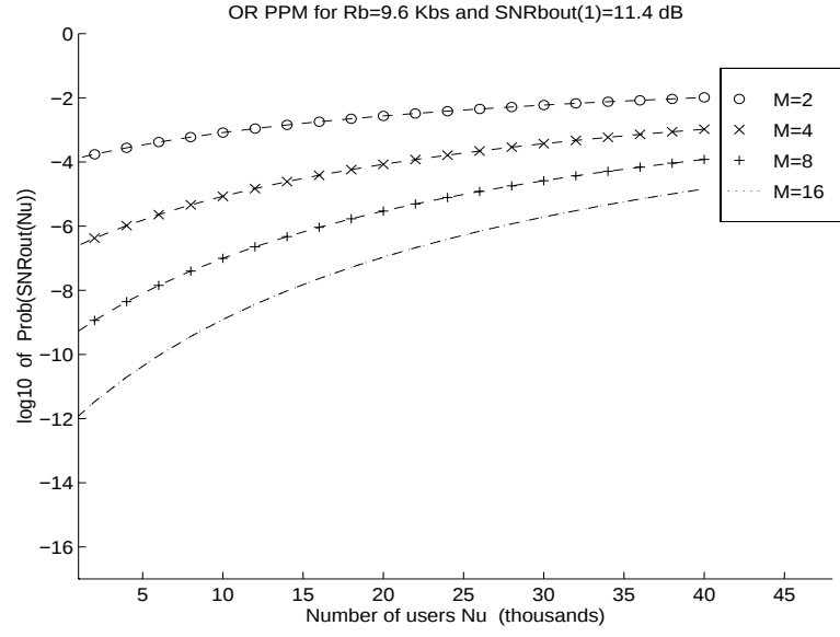
Figure 5.2: The base 10 logarithm of the probability of bit error for OR PPM signals, as a function of N_u for different values of M , using R_b = 9.6 Kbps, \text{SNRb}_{\text{out}}^{\text{OR}}(1) = 11.40 dB and set 1 of parameters in table 5.1.
