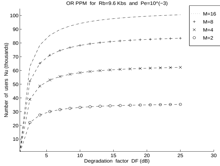
Figure 5.12: The number of users N_u(\text{DF}) for OR PPM signals, calculated for different values of M under perfect power control conditions using R_b = 9.6 Kbps, P_e = \text{UBP}_b^{\text{OR}}(1) \simeq 10^{-3} and set 1 of parameters in table 5.1.
