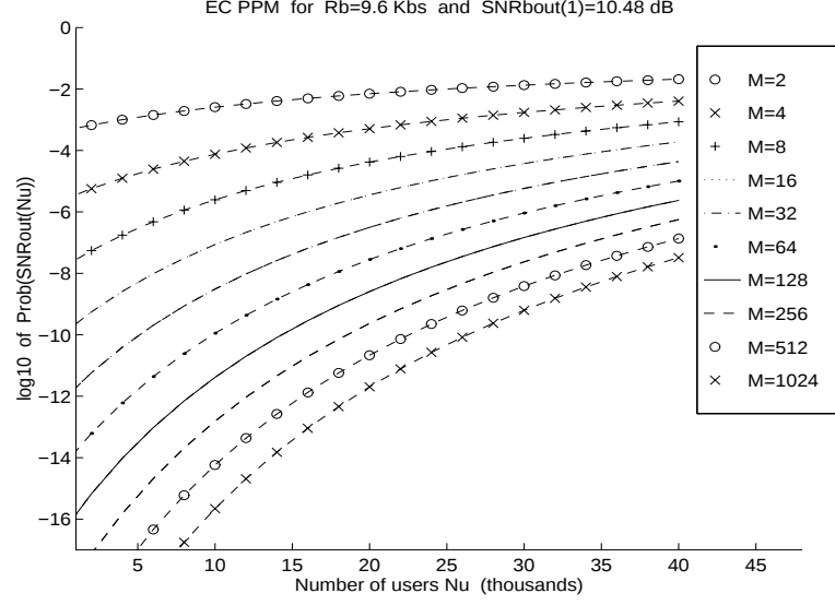
Figure 5.1: The base 10 logarithm of the probability of bit error for EC PPM signals, as a function of the number of simultaneous users N_u for different values of M , using R_b = 9.6 Kbps, \mathbf{SNRb}_{\text{out}}^{\text{BC}}(1) = 10.48 dB and set 1 of parameters in table 5.1.
