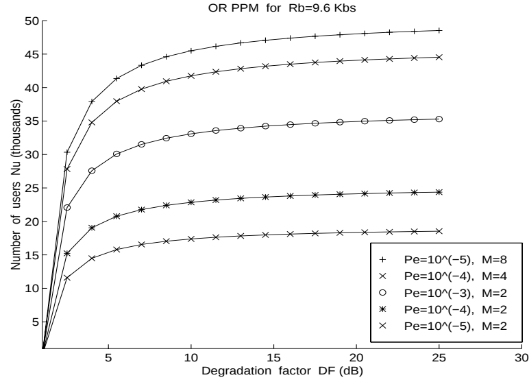
Figure 5.13: The number of users N_u(\text{DF}) for OR PPM signals calculated for different pairs (M, P_e) , with P_e = \text{UBP}_b^{\text{OR}}(1) . The curves were calculated using R_b = 9.6 Kbps and set 1 of parameters in table 5.1.
