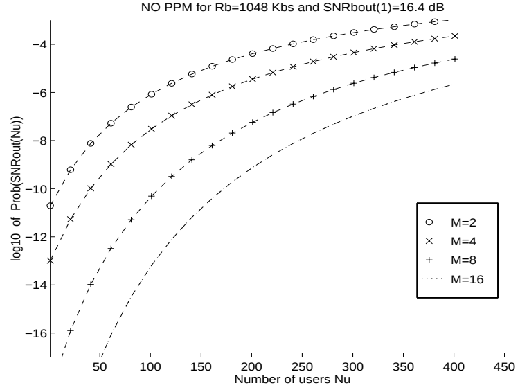
Figure 5.9: The base 10 logarithm of the probability of bit error for NO PPM signals, as a function of N_u for different values of M , using R_b = 1048 Kbps, \text{SNR}_{\text{out}}^{\text{MTSK}(1,2)}(1) = 16.40 dB, \text{SNR}_{\text{out}}^{\text{OR}}(1) = 14.30 dB and set 1 of parameters in table 5.1.
