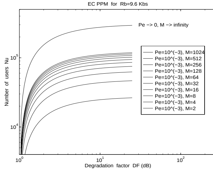
Figure 5.14: The number of users N_u(\text{DF}) for EC PPM signals, calculated using 2 \leq M \leq 1024 with P_e = \text{UBP}_b^{\text{EC}}(1) \simeq 10^{-3} . Also shown is the value of N_u(\text{DF}) \rightarrow N_{\text{IR}} for large values of both DF and M . The curves were calculated using R_b = 9.6 Kbps and set 1 of parameters in table 5.1.
