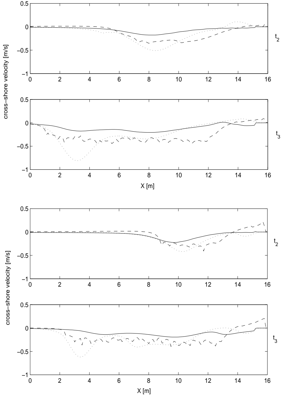
FIGURE 9. Cross-shore velocity computed at the cross-shore section of the rip channel (section D) for bathymetry (b) (upper panels) and (c) (lower panels). Results from a wave-averaged simulation run with SHORECIRC (dotted line), from a wave-resolving simulation run with FUNWAVE2D (solid line) and from the dissipative PV model (dashed line), are plotted for the two steps t_2 and t_3 of evolution.
