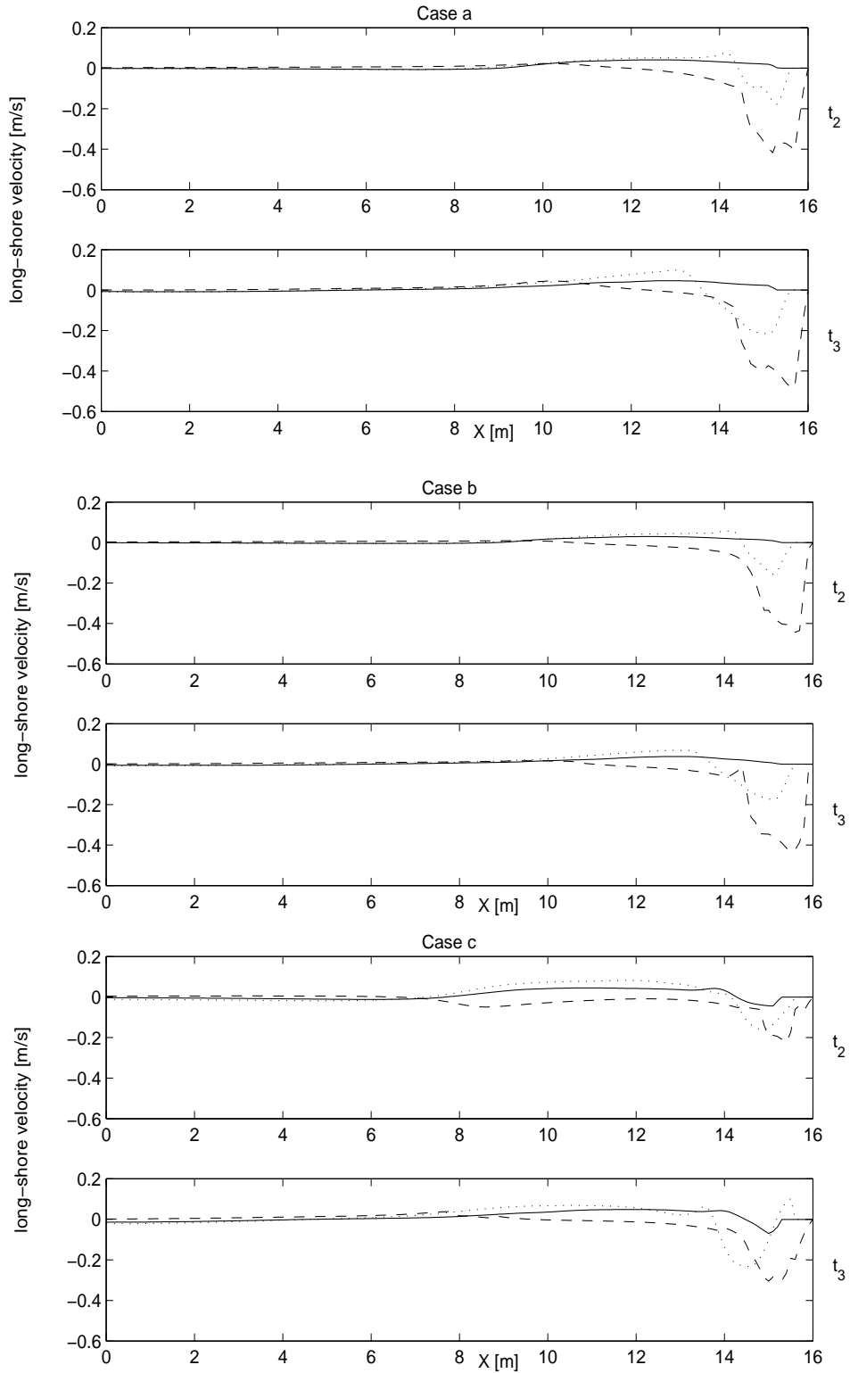
FIGURE 10. Longshore velocity computed at the cross-shore section E outside the rip channel of figure 5. Results from a wave-averaged simulation run with SHORECIRC (dotted line), from a wave-resolving simulation run with FUNWAVE2D (solid line) and from the viscous PV model (dashed line), are plotted together at the steps t_2 (top panel) and t_3 (middle panel) of evolution.
