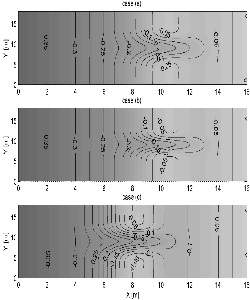
FIGURE 3. Rip bathymetries obtained from equation (5.3). Case (a): bathymetry obtained with x_{ba} = 10m , M = 0.1 , \sigma = 2 and a = 3 ; case (b): bathymetry with a narrower rip-channel ( a = 2 ); case (c): bathymetry with the bar moved offshore ( x_{ba} = 8m ) but with the same freeboard ( M = 0.15 , \sigma = 2 and a = 3 ).
