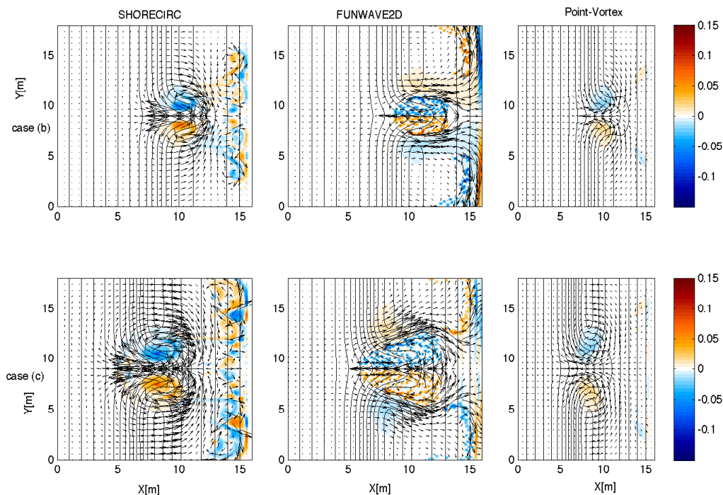
FIGURE 7. Velocity and vorticity fields predicted by the models under analysis for the stage t_2 flow. Top panel: bathymetry (b). Bottom panel: bathymetry (c). For graphical arrangements see figure 6.
