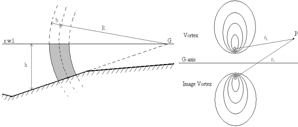
FIGURE 1. The virtual extension of the vortex tube to a three-dimensional vortex ring of radius R (left panel) and streamlines for a vortex and its image, distances r_1 and r_2 to the point P (right panel).
