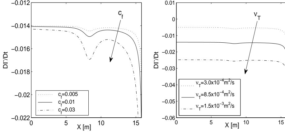
FIGURE 4. D\Gamma/Dt evaluated for given vortex size in the case of the rip current bathymetry (a). Left panel: cross-shore profile of D\Gamma/Dt for fixed eddy viscosity ( \nu_T = 8.5 \times 10^{-4} \text{ m}^2/\text{s} ) and for different values of the friction factor. Right panel: cross-shore profile of D\Gamma/Dt for fixed friction factor ( c_f = 0.01 ) and for different values of the eddy viscosity.
