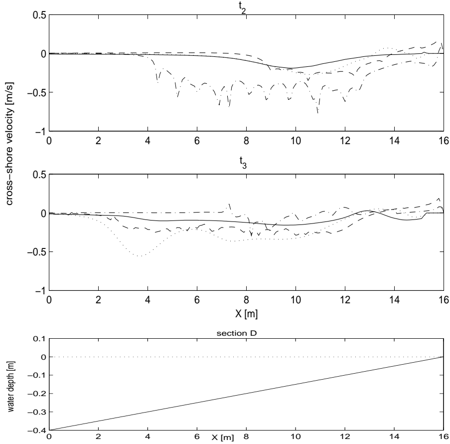
FIGURE 8. Cross-shore velocity computed at the cross-shore section D of figure 5 of the rip channel. Results from a wave-averaged simulation run with SHORECIRC (dotted line), from a wave-resolving simulation run with FUNWAVE2D (solid line) and from the dissipative PV model (dashed line) and from the inviscid PV model (dash-dotted line), are plotted for the two steps t_2 (top panel) and t_3 (middle panel) of evolution. The bottom panel reports, for reference, the bathymetry of the chosen section.
