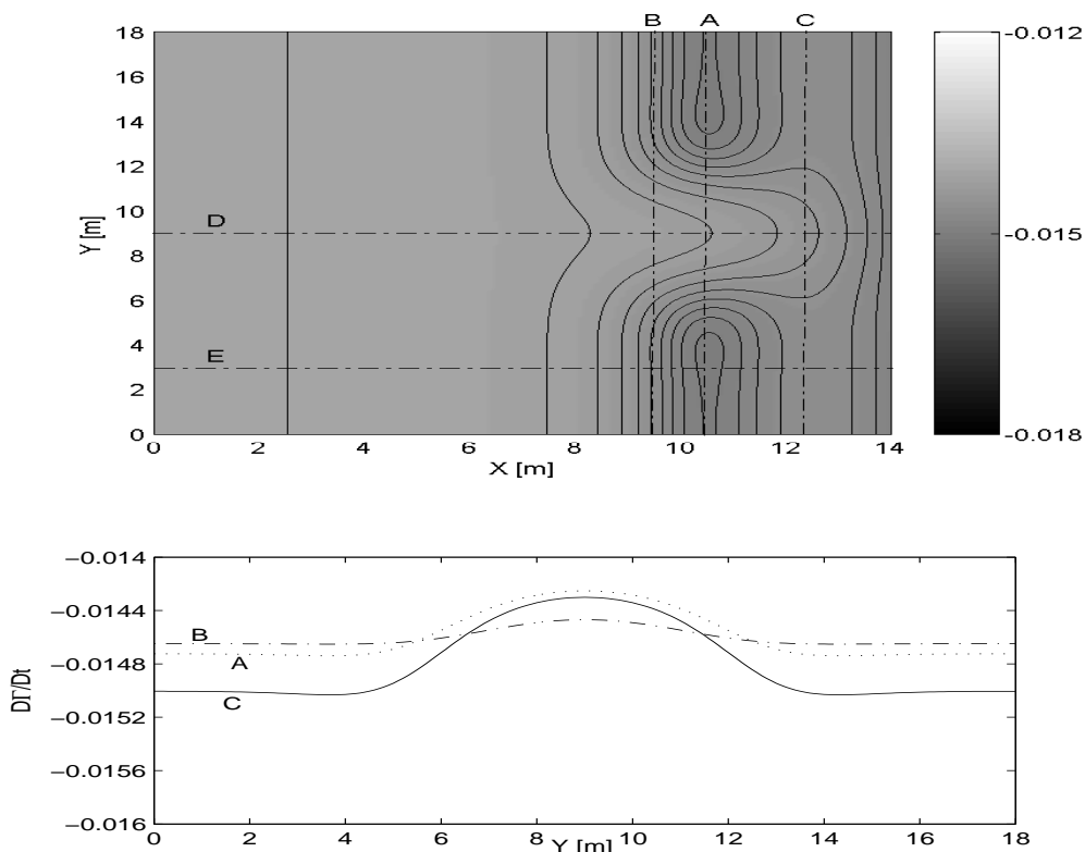
FIGURE 5. D\Gamma/Dt of equation (3.21) evaluated for given vortex size in case of the rip current bathymetry (a) of figure 3 with c_f = 0.01 and \nu_T = 8.5 \times 10^{-4} \text{ m}^2/\text{s} : the complete spatial distribution (top panel) and three longitudinal sections (bottom panel), over the bar crest A, (solid line), offshore of the bar B, (dash-dotted line), and shorewards of the bar C, (dotted line).
