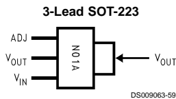
DS009063-59 Front View Order Part Number LM317EMP or LM317AEMP Package Marked N01A See NSC Package Number MA04A
