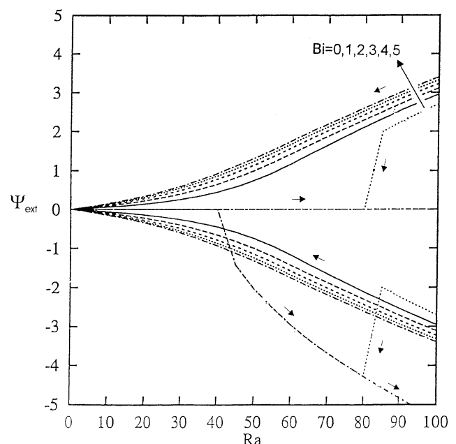
Fig. 2. \psi_{\text{ext}} as a function of the Darcy–Rayleigh number obtained using Bi numbers from 0 to 5.
