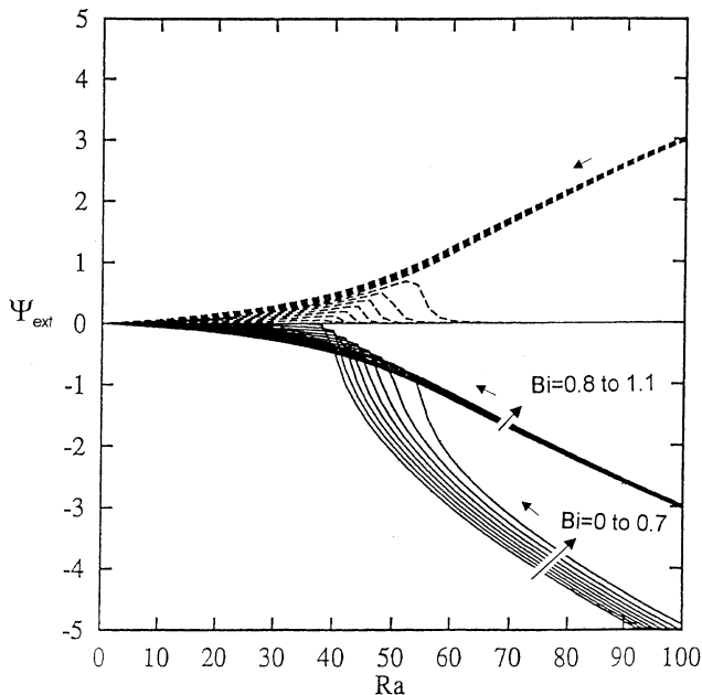
Fig. 3. \psi_{\text{ext}} as a function of the Darcy–Rayleigh number and various Bi numbers at the decreasing branch. The initial conditions for all the cases are from the steady-state solutions obtained at Ra = 400 , Bi = 0 with unicellular flow. The symmetrical upper and lower branches are with Bi = 0.8 \rightarrow 1.1 . Non-symmetrical upper and lower branches are for Bi = 0 \rightarrow 0.7 .
