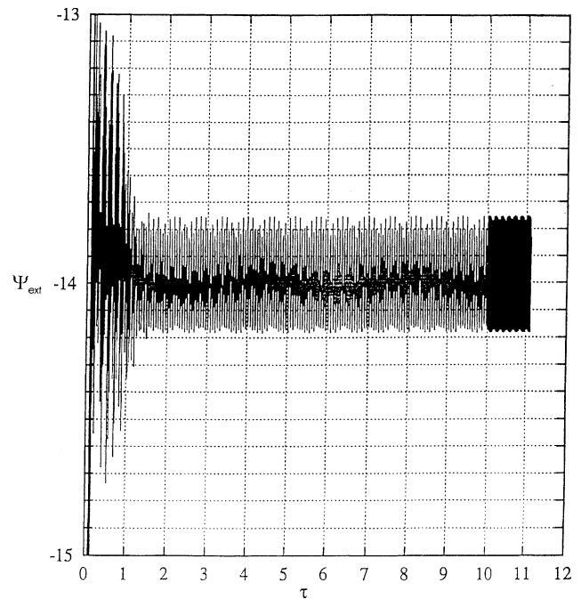
Fig. 5. \psi_{\text{ext}} as a function of time for the case of Ra = 400 and Bi = 0 . The initial condition is with Ra = 100 and unicellular flow.
