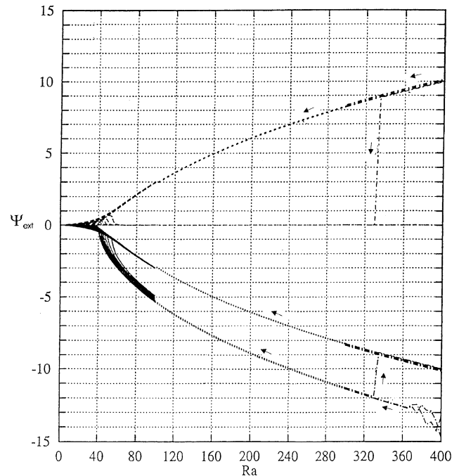
Fig. 4. \psi_{\text{ext}} as a function of the Darcy–Rayleigh number and various Bi numbers at the lower branch. The initial conditions are the same as for Fig. 3.
