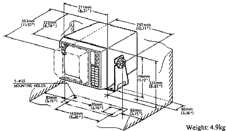
Fig.10 Display Unit Outline Drawing
