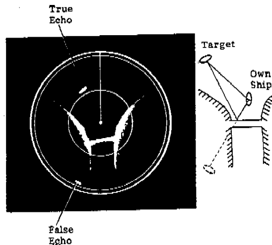
Fig.35 Indirect Echoes
