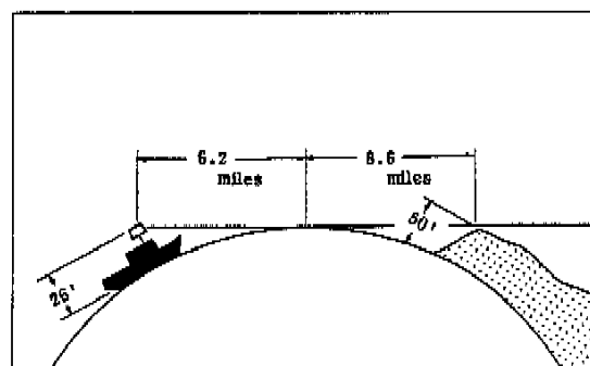
Fig.30 Radar Horizon
