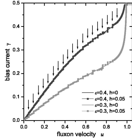
FIG. 4. The numerically simulated \gamma - u curves in the presence of magnetic field h=0.05 . The amplitude of ac drive was chosen \varepsilon=0.3 and 0.4 , and other parameters are the same as in Fig. 1. Arrows identify Shapiro steps.
