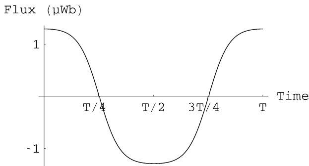
Fig. 4. Cut flux for an excitation of the string Y_I = 10 mm along y . String altitude: d = 5 mm. Magnet position L/4 : neck pickup.
