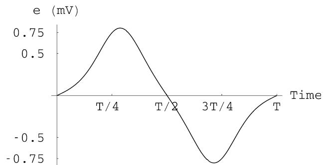
Fig. 6. Electromotive force for an excitation of the string Y_I = 6 mm along y , string initially shifted of 3 mm. String altitude: d = 5 mm. Magnet position L/4 : neck pickup.
