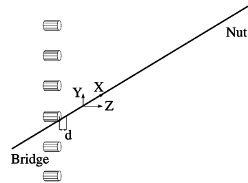
Fig. 1. Pickup geometry: the six magnets and one string. The coil is wound around the six magnets and is not represented here.
