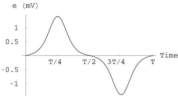
Fig. 5. Electromotive force for an excitation of the string Y_I = 10 mm along Oy . String altitude: d = 5 mm. Magnet position L/4 : neck pickup.
