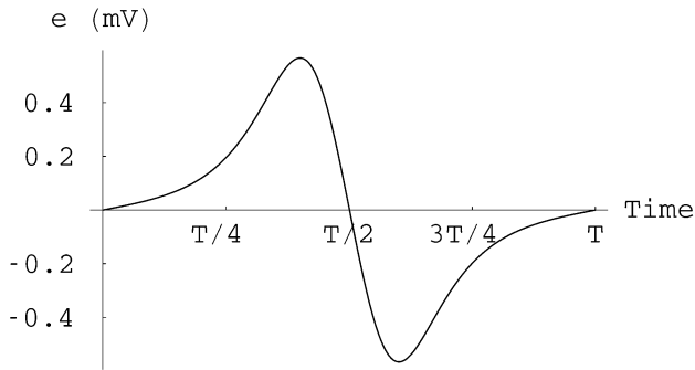
Fig. 7. Electromotive force for an excitation of the string Z_I = 6 mm along z . String altitude: d = 5 mm. Magnet position L/4 : neck pickup.
