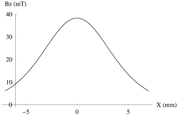
Fig. 2. z component of the magnetic flux density for a circular section of 4.5 mm diameter along the x axis at a distance d = 5 mm along z above the magnet.
