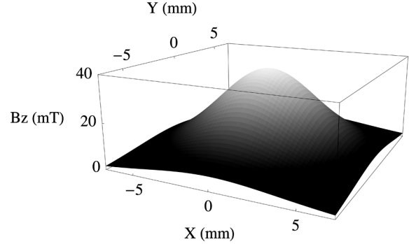
Fig. 3. B_z component of the flux density above the square section magnet. Altitude: d = 5 mm.
