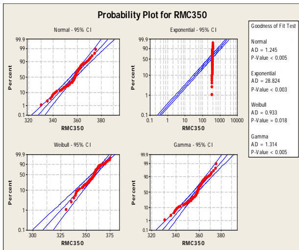
Figure 3 – Probability Plots for the Concrete Compressive Strength
