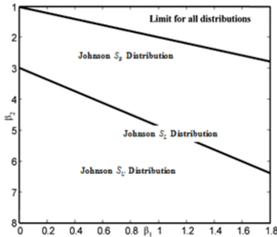
Figure (1): The Skewness and Kurtosis Plane for the Johnson Distributions
