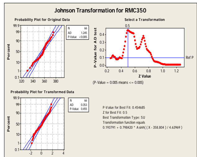
Figure 4 – Probability Plots for the Johnson Transformed data of Concrete Strength
