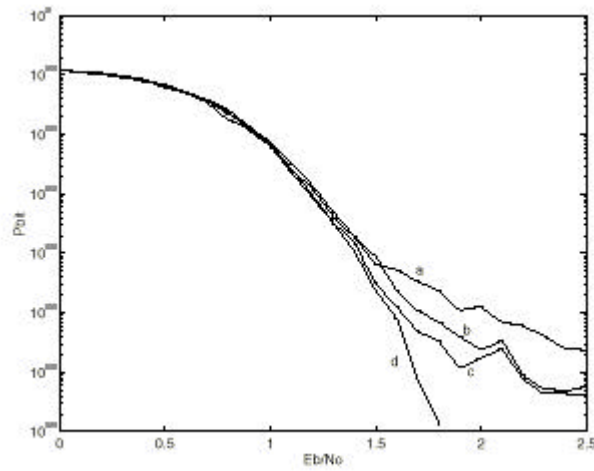
Figure 4. Convergence of “constellation” interleaver for PCCC
