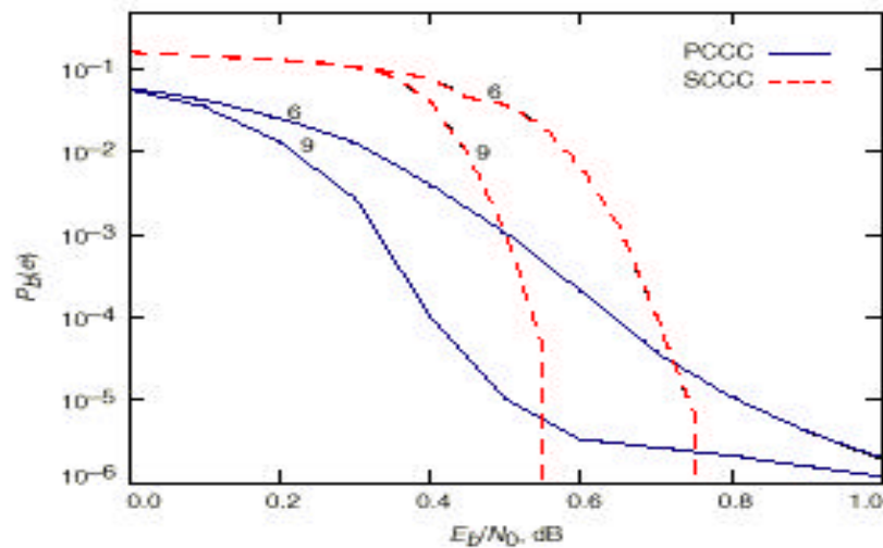
Figure 10. Comparison between PCCC and SCCC techniques.
