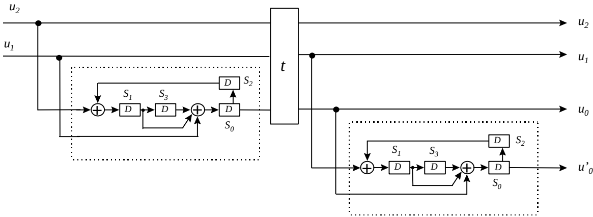
Figure 6. Serial Convolutional Concatenated Encoders
