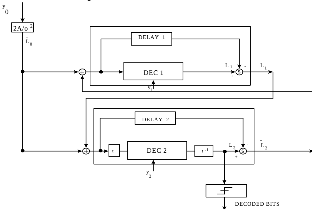
Figure 3.- PCCC Decoder
