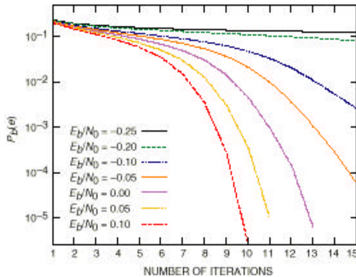
Figure 9. Convergence of iterative decoding for SCCC using ASW-SISO algorithm
