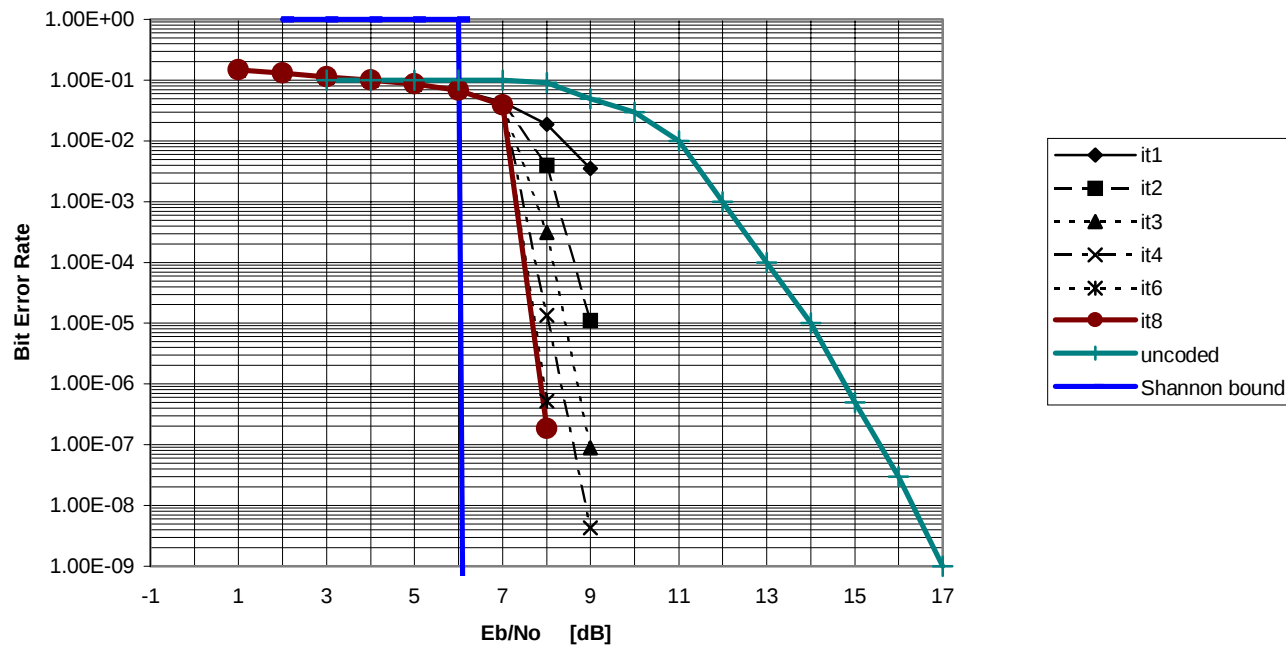
BER for Rate 4/6 64QAM N=10400 bits AWGN Channel
