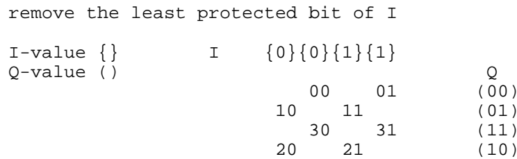
Figure 5. 8 QAM case 2.
