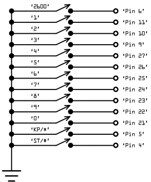
'KEYPAD TO PROM PIN ASSIGNMENTS'
