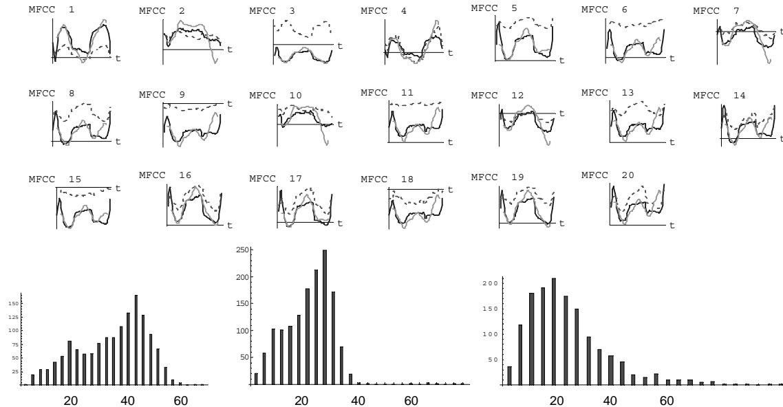
Figure 3: Upper: The solid blue and dashed red lines show the MFCCs of the clean and corrupted versions of the words “and make”, respectively, after “normalization” by CMN. The solid green line shows the corrupted MFCCs after the new channel conversion procedure. Lower: The distribution of Euclidean distances between the corrupted and clean cepstra after CMN (left), after CMN + SS (center), and after the new channel conversion process (right). The means (99% confidence intervals) of these distributions are: 35.4+0.9, 22.9+0.6, and 23.4+1.0.
