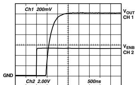
TPC 13. Power-Up Response Time
