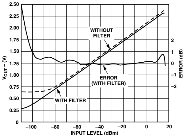
Figure 23. Results for 120 dB Measurement System
