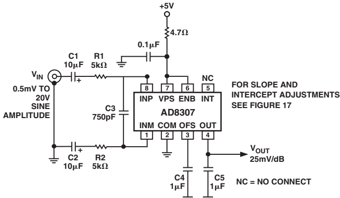
Figure 24. Connections for Low Frequency Operation
