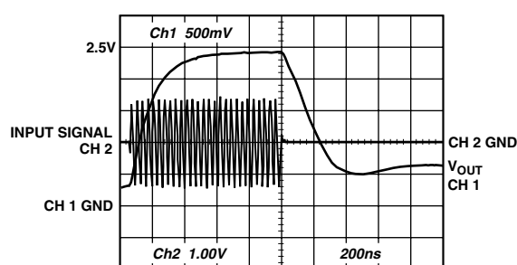
TPC 17. Large Signal Response Time
