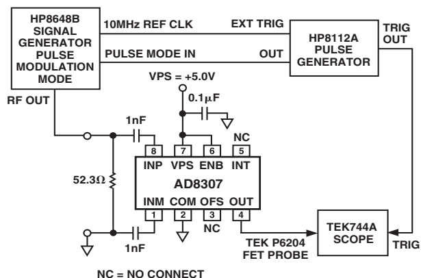
TPC 18. Test Setup for V_{OUT} Pulse Response
