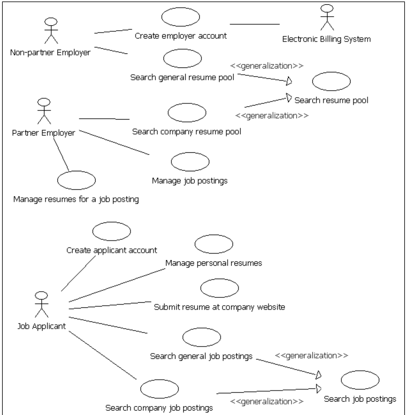
Figure 1: DISTRIMON Use Case Diagram
