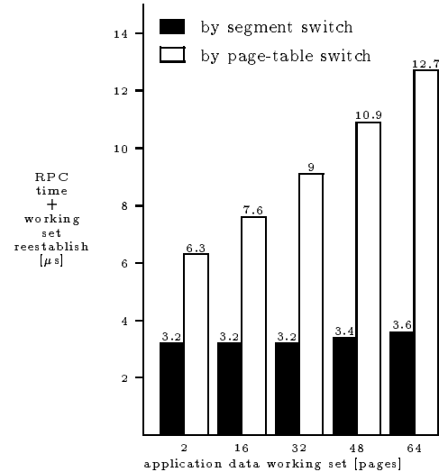
Figure 2: Segmented Versus Standard Address-Space Switch in L3 on Pentium, 90 MHz.
