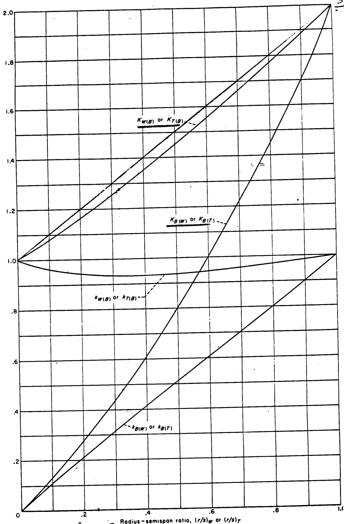
Figure 7 Values of lift ratios based on slender-body theory.
