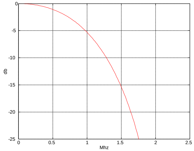
CHRBW = '0'
