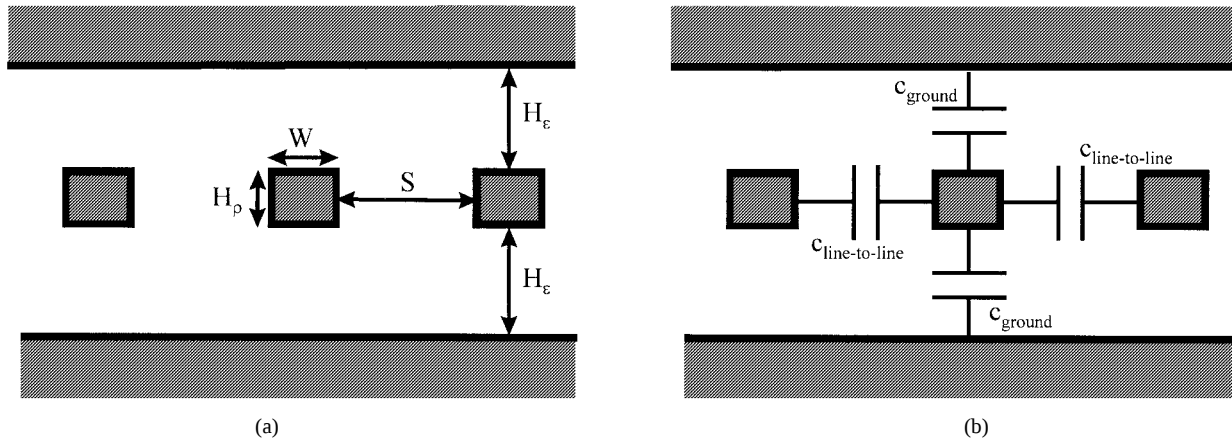
Fig. 3. The definition of (a) the interconnect dimensions and (b) the capacitive components.
