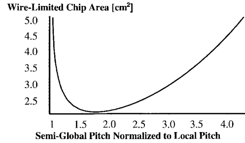
Fig. 7. Wire-limited chip area versus semiglobal pitch.
