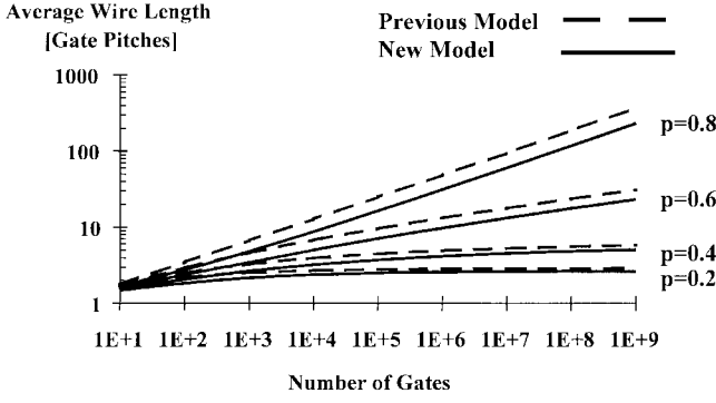
Fig. 1. Average interconnect length versus number of gates for p = 0.2, 0.4, 0.6 , and 0.8 .
