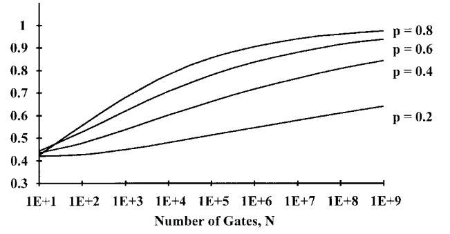
Fig. 2. Longest interconnect length normalized to twice the chip edge versus number of gates for p = 0.2, 0.4, 0.6 , and 0.8 .
