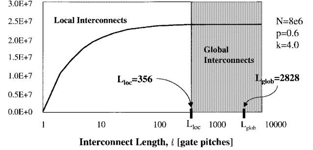
Fig. 5. The c.i.d.f. for a system with a two-tier multilevel architecture.
