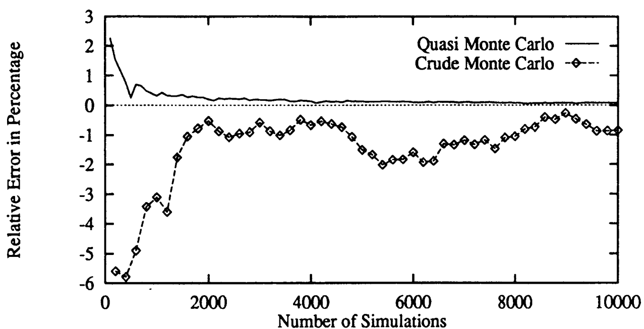
Figure 5 Standard European Call Option (Delta)
