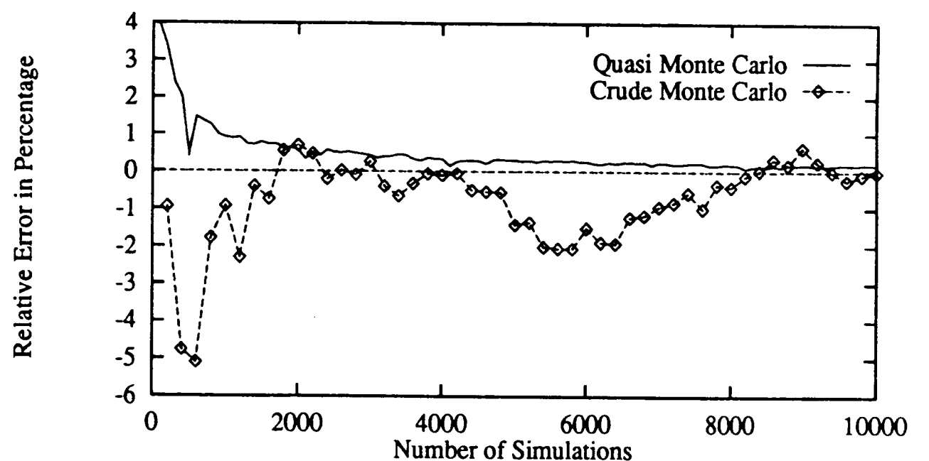
Figure 3 Standard European Call Option
