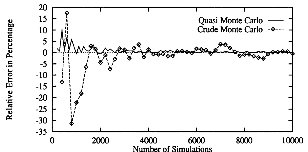
Figure 6 Standard European Call Option (Gamma)
