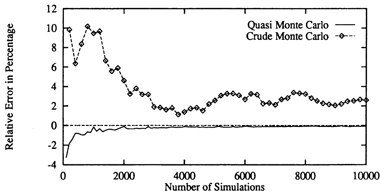
Figure 4 Standard European Put Option
