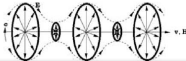
Figure 1. Electric ring vortices form a magnetic wave.
