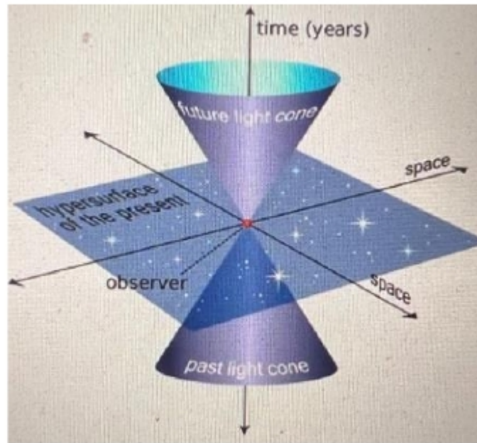
Figure 1: How Scalar Waves Propagate
