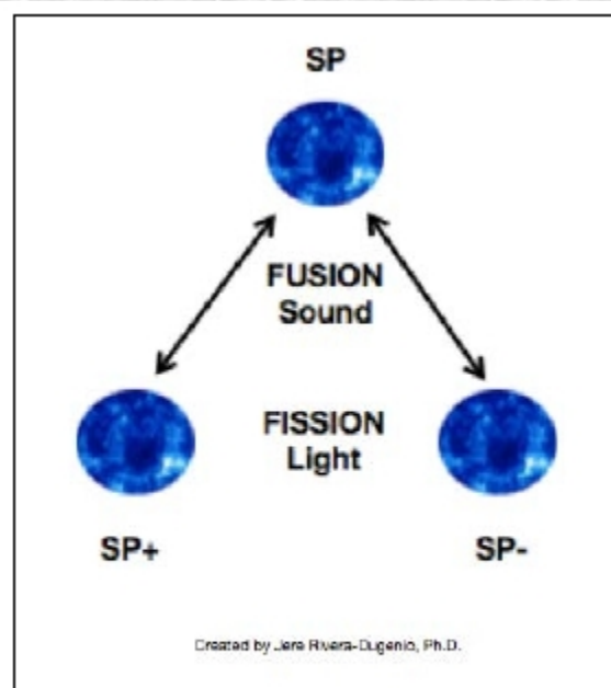
Figure 2. The Perpetual Fission-Fusion Scalar Wave
