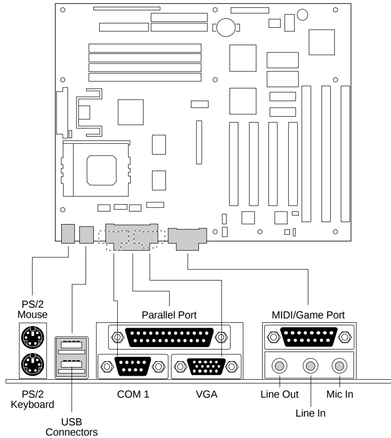
Figure 5. Back Panel Connectors
