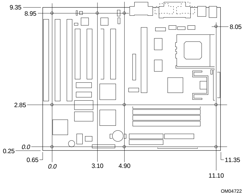
Figure 2. Board Dimensions
