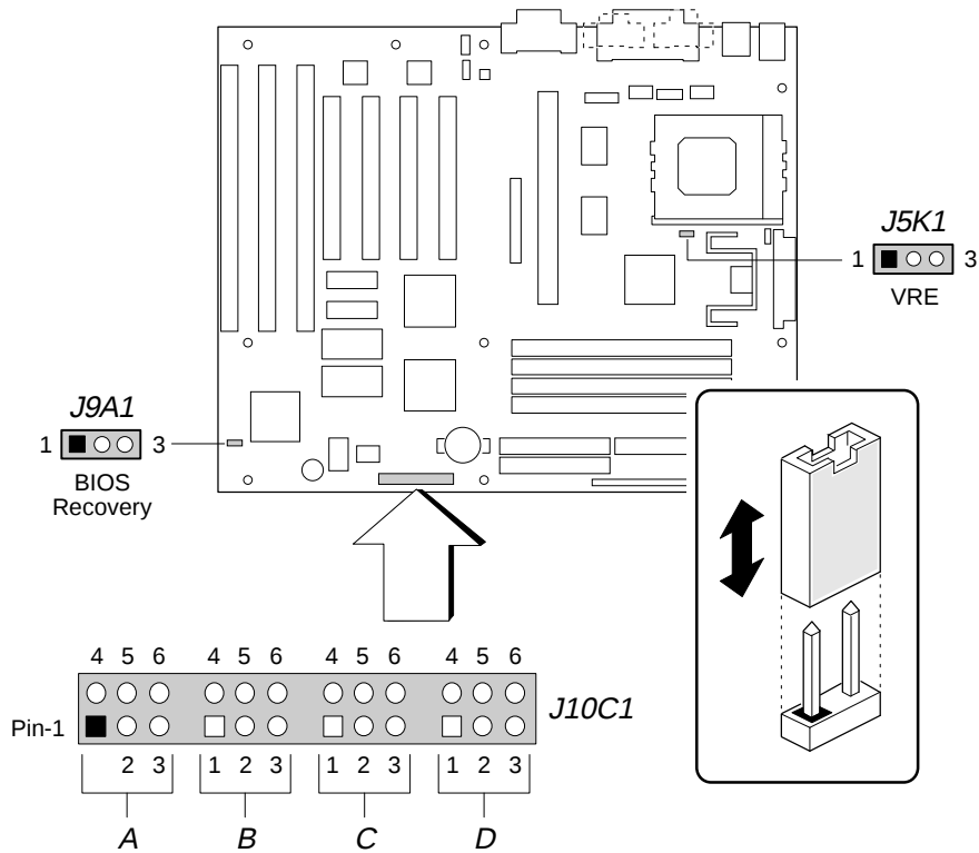
Figure 6. Jumper Locations
