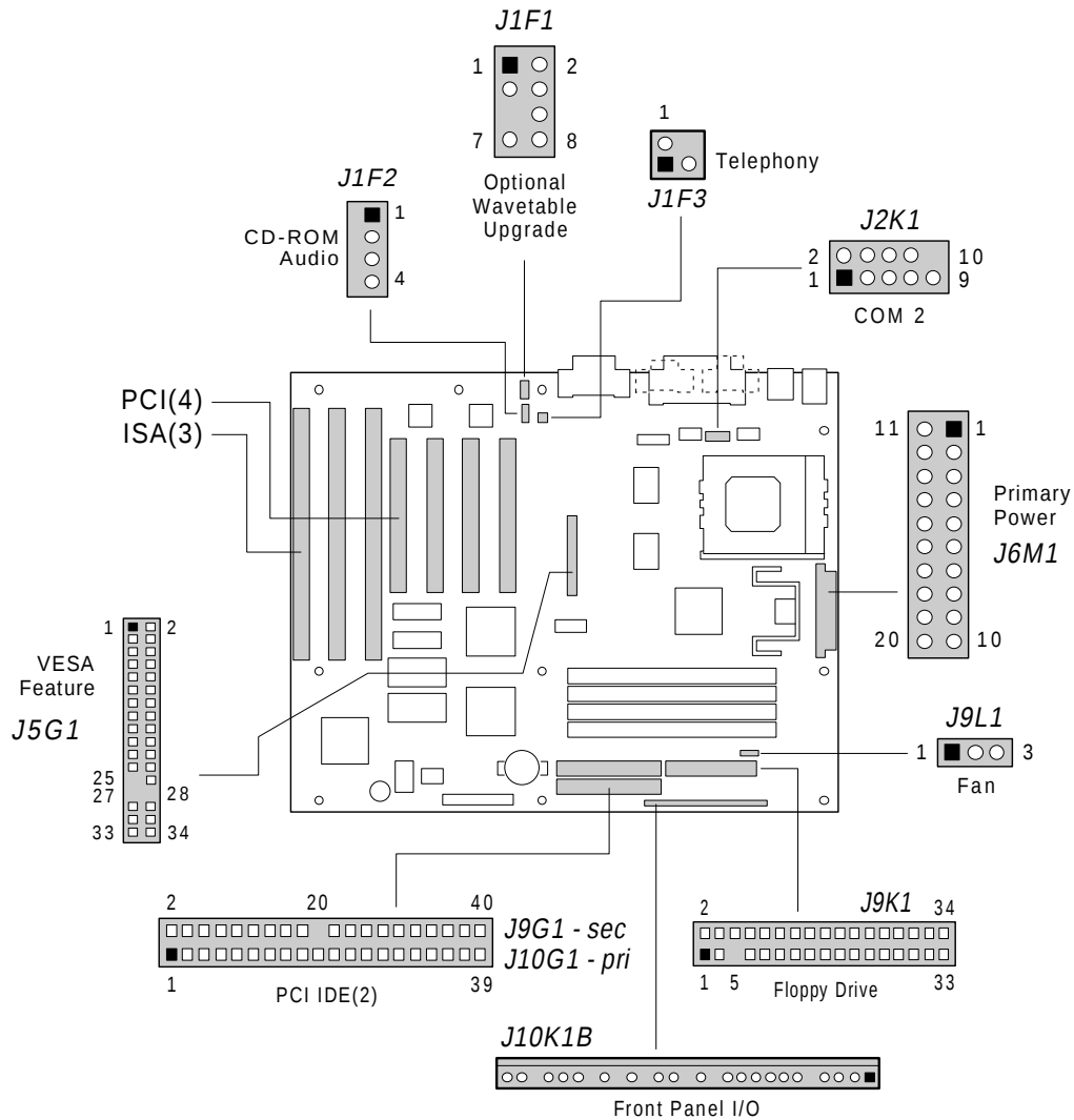
Figure 3. Motherboard Connector Locations
